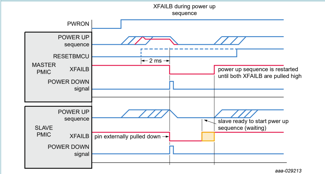
Figure 21. External XFAILB event during a power up sequence
