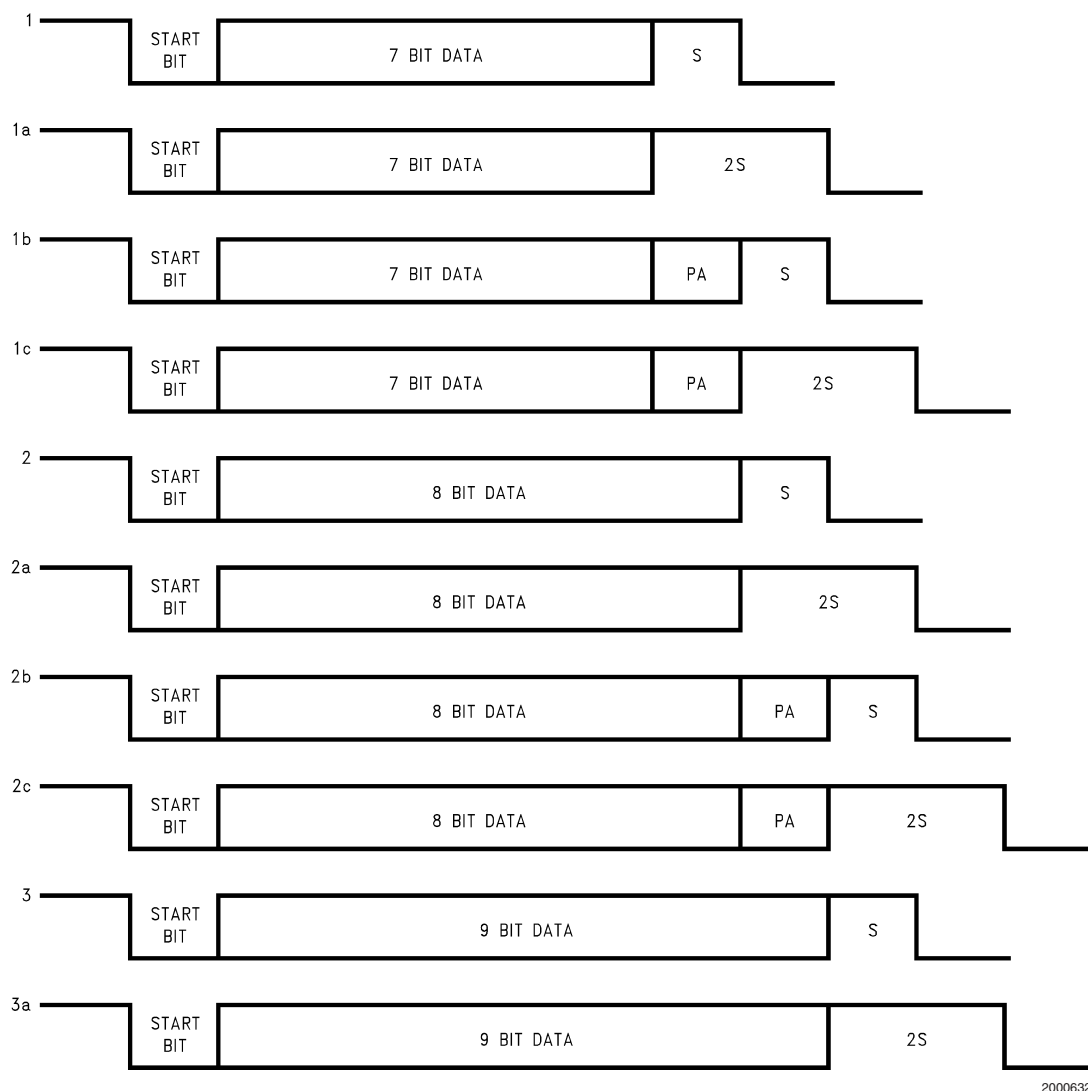
FIGURE 22. Framing Formats
