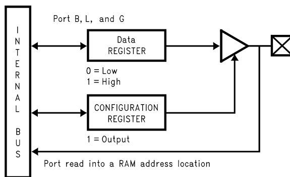
FIGURE 3. I/O Port Configurations—Output Mode
