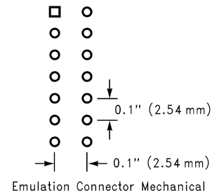
FIGURE 5. Emulation Connection
