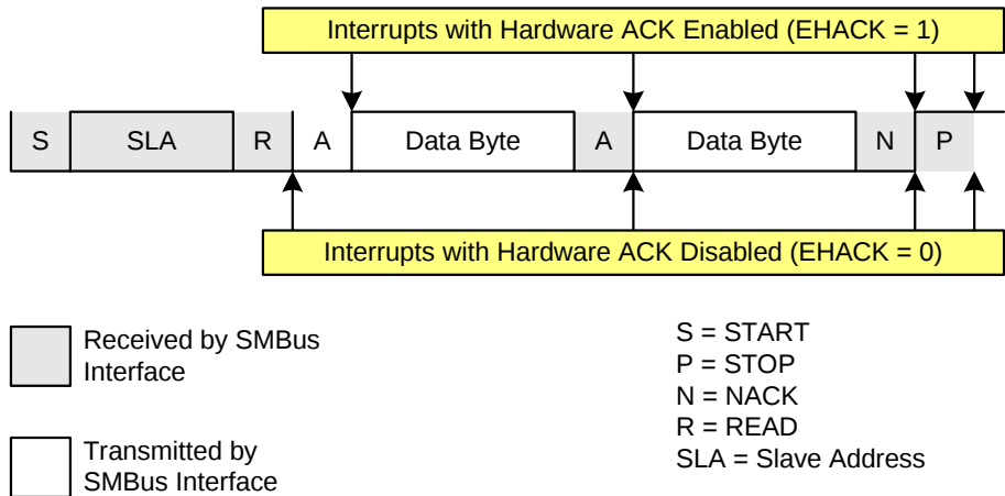
Figure 21.8. Typical Slave Read Sequence
