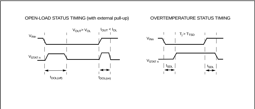
Figure 4. Status timing
