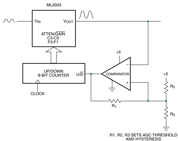
Figure 16. Analog AGC
