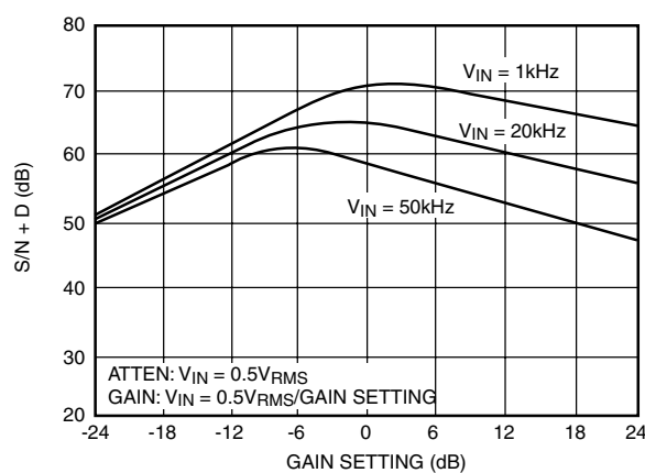
Figure 9. S/N + D vs Gain Setting ( V_{IN}/V_{OUT} = 0.5\text{VRMS} )
