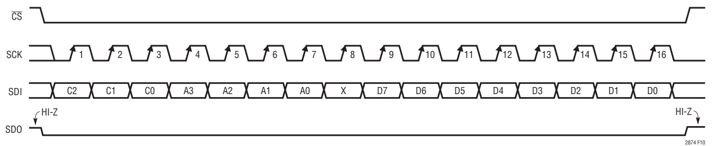
Figure 10. SPI Interface Timing (Write or WrtUpd)
