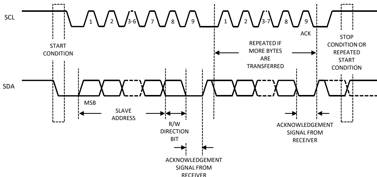
Figure 7. Data Transfer on I²C Serial Bus
