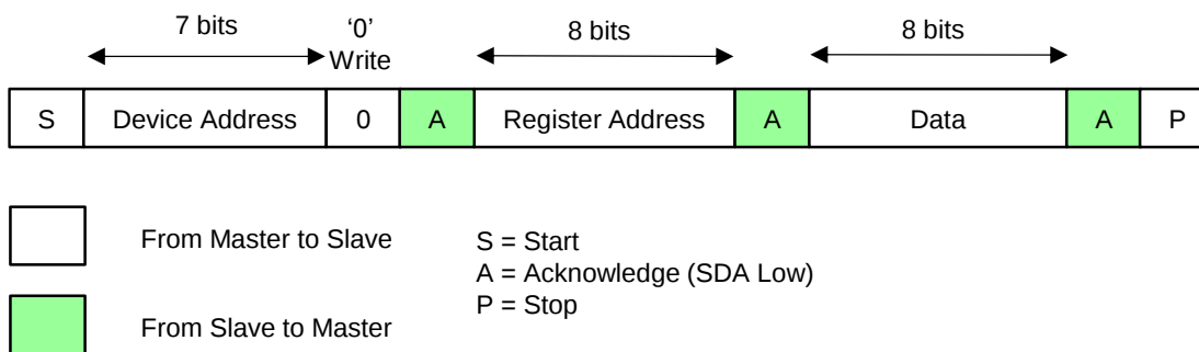
Figure 8. I²C Write Cycle
