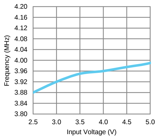
Switching Frequency vs. VIN
