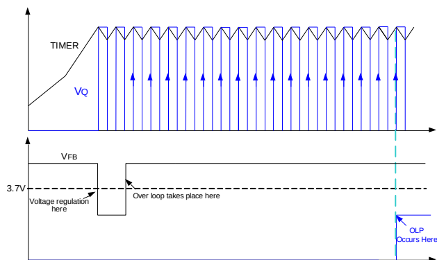
Figure 8: Overload Protection
