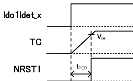
Fig.7.2 Power-on reset
