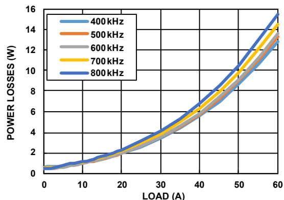
FIGURE 11. ISL99227, ISL99227B POWER DISSIPATION ( V_{IN} = 12\text{V} ; V_{OUT} = 1.8\text{V} ; L_{OUT} = 0.18\mu\text{H}/0.17\text{m}\Omega/\text{FP1008-180-R} )
