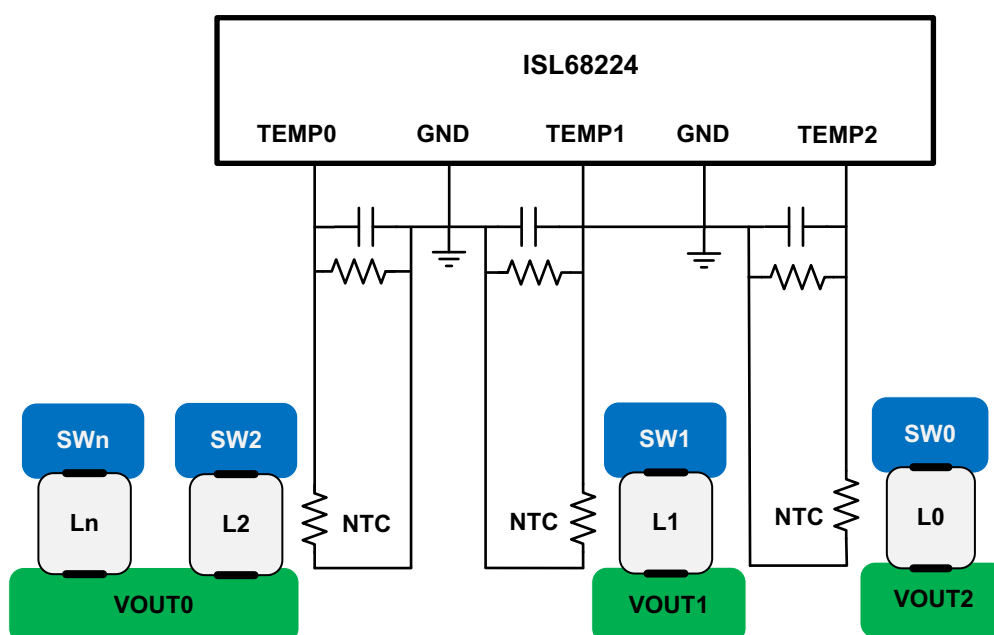
Figure 16. NTC Placement
