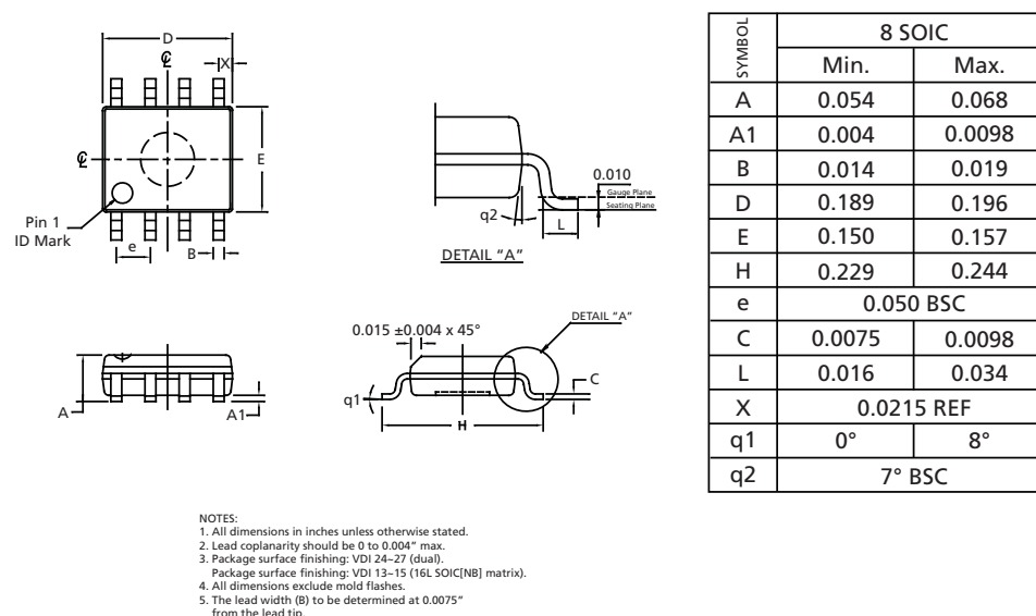
Figure 5-1: Package Dimensions
