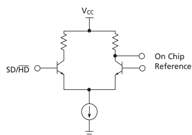
Figure 2-4: Slew Rate Select Input Stage (SD/ \overline{\text{HD}} )
