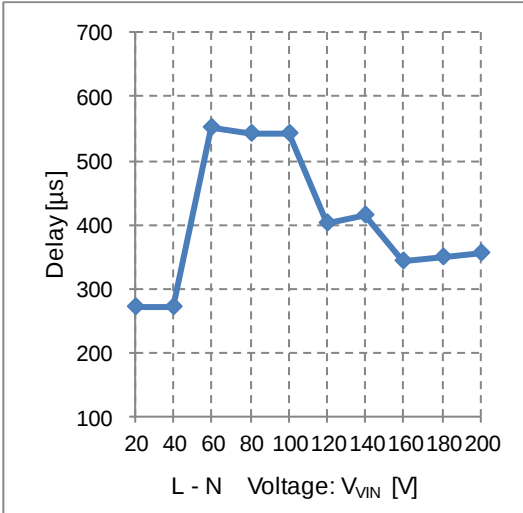
Figure 24. Delay vs L – N Voltage (The reference data at the normal voltage rectification)
