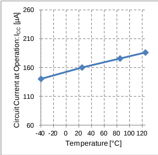
Figure 12. Circuit Current at Operation vs Temperature
