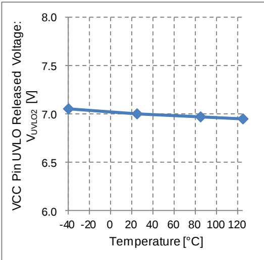
Figure 14. VCC Pin UVLO Released Voltage vs Temperature
