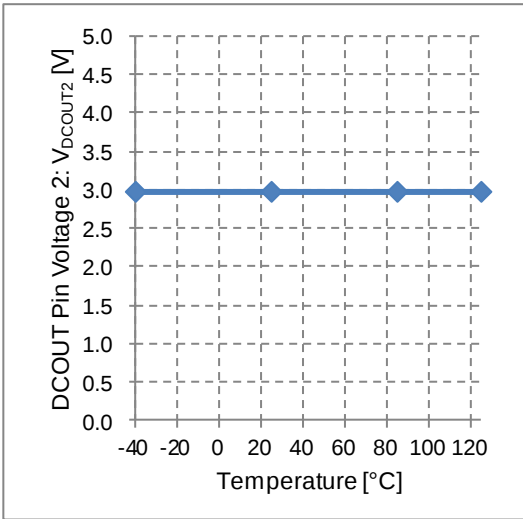
Figure 22. DCOUT Pin Voltage 2 vs Temperature
