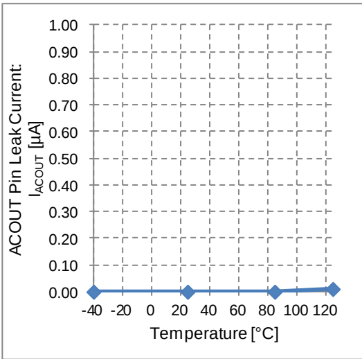
Figure 18. ACOUT Pin Leak Current vs Temperature
