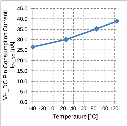
Figure 20. VH_DC Pin Consumption Current vs Temperature
