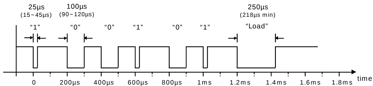
FIGURE 17. 1-WIRE INTERFACE
