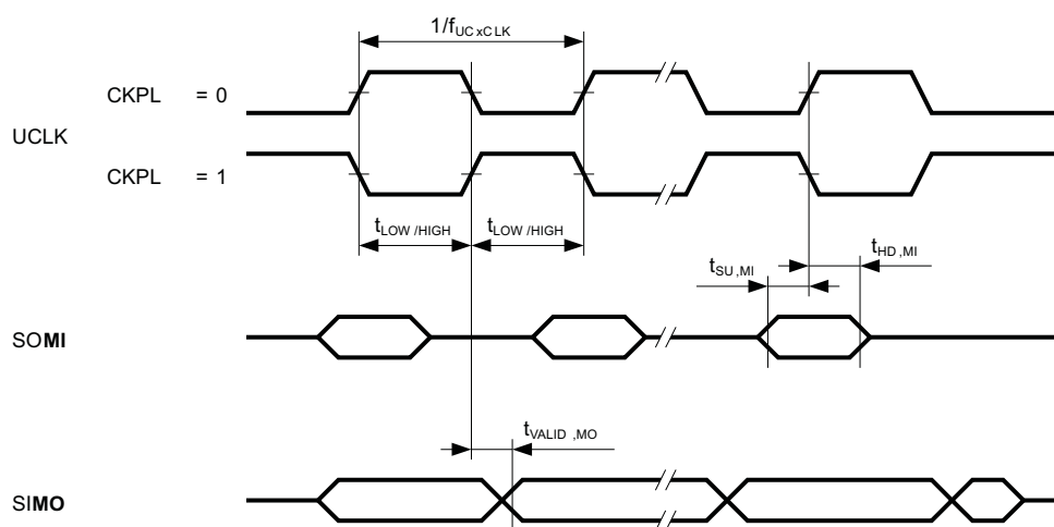
Figure 5-32. SPI Master Mode, CKPH = 1
