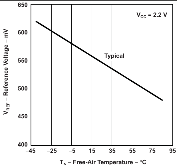
Figure 5-16. Reference Voltage vs Free-Air Temperature
