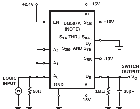
FIGURE 1B. DG507A TEST CIRCUIT
