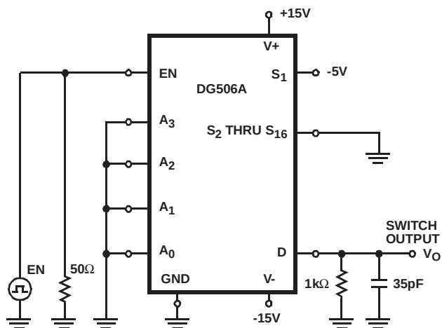
FIGURE 2A. DG506A TEST CIRCUIT
