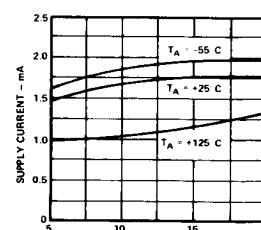
Supply Current
