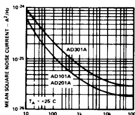
Input Noise Current
