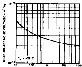
Input Noise Voltage
