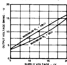
Output Swing
