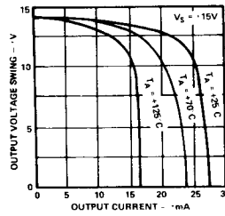
Current Limiting
