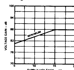
Voltage Gain
