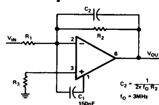
Figure 3. Feedforward Compensation
