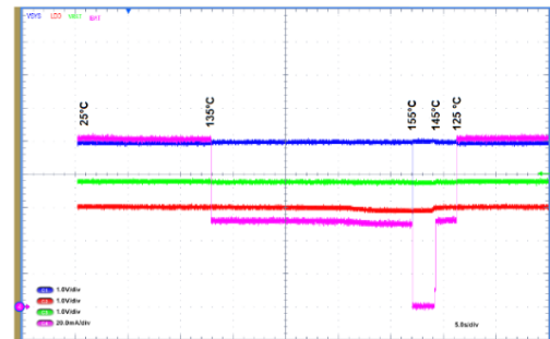
Figure 4. Thermal management
