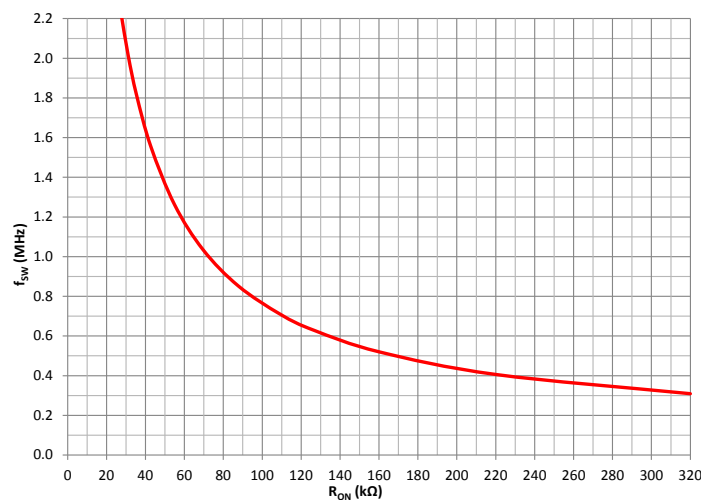
Figure 6: Average Switching Frequency versus R_{ON} Resistance ( V_{IN} = 12 \text{ V} , V_{OUT} \approx 7 \text{ V} , i_{LED} = 1 \text{ A} )
