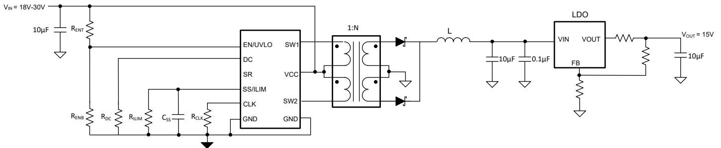
Figure 9-4. Typical Application Schematic for Wide-Ranging Input with Duty Cycle Control
