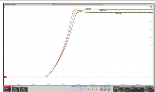
Figure 6-12. Output Voltage During Soft Start with 50-mA, 250-mA, and 500-mA Loads SN6507-Q1 + Würth 750319696 V_{IN} = 24\text{ V} R_{ILIM} = 18.2\text{ k}\Omega C_{SS} = 50\text{ nF}
