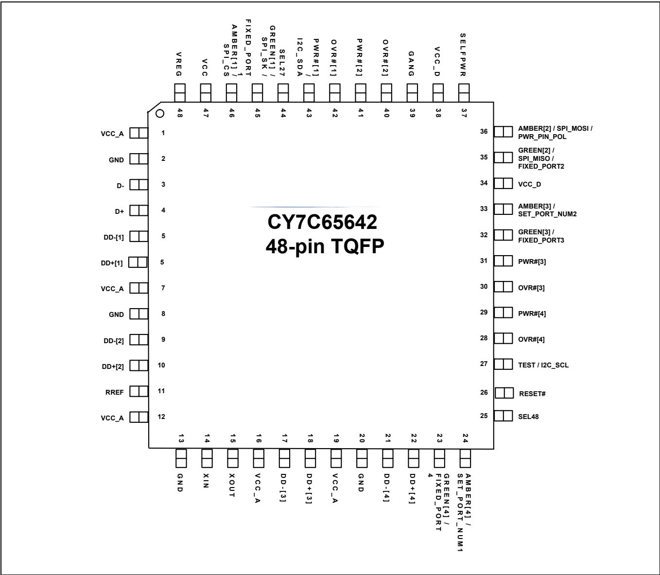
Figure 4 48-pin TQFP (7 × 7 × 1.4 mm) pinout
