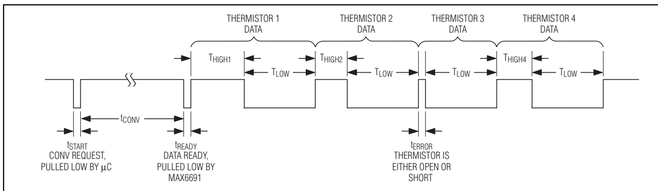
Figure 1. Timing Diagram
