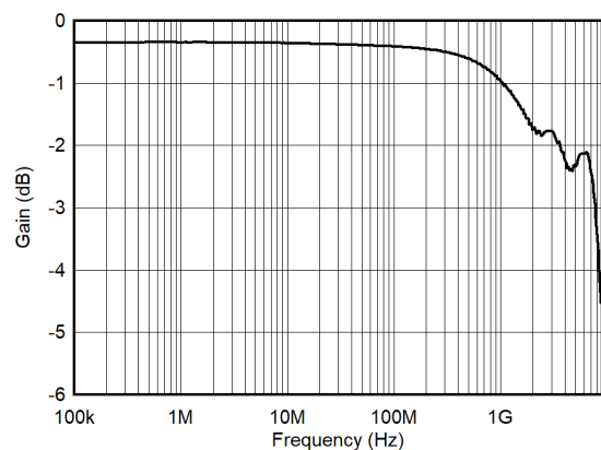
Figure 6-15. Differential Bandwidth
