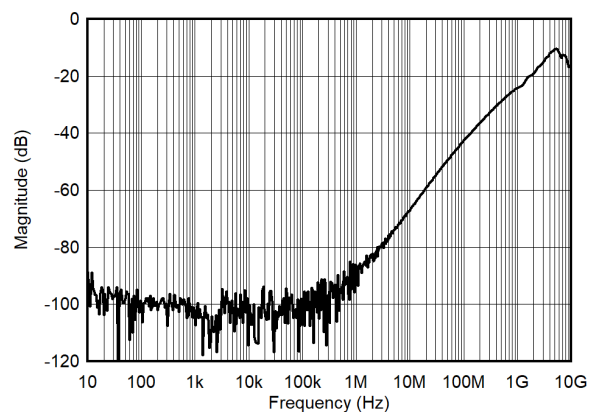
Figure 6-16. Off Isolation
