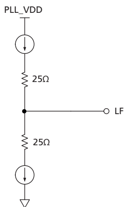
Figure 3-7: Loop Filter (LF)
