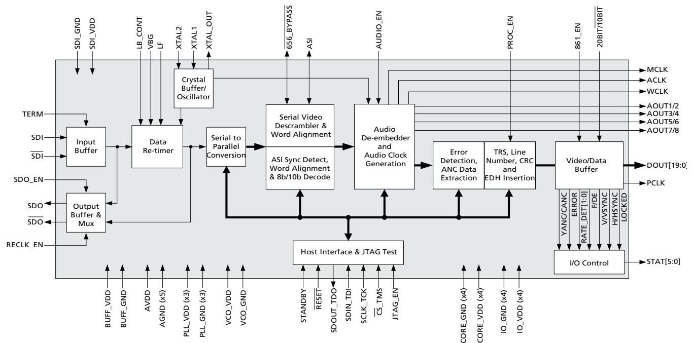
Figure A: GV7605 Functional Block Diagram
