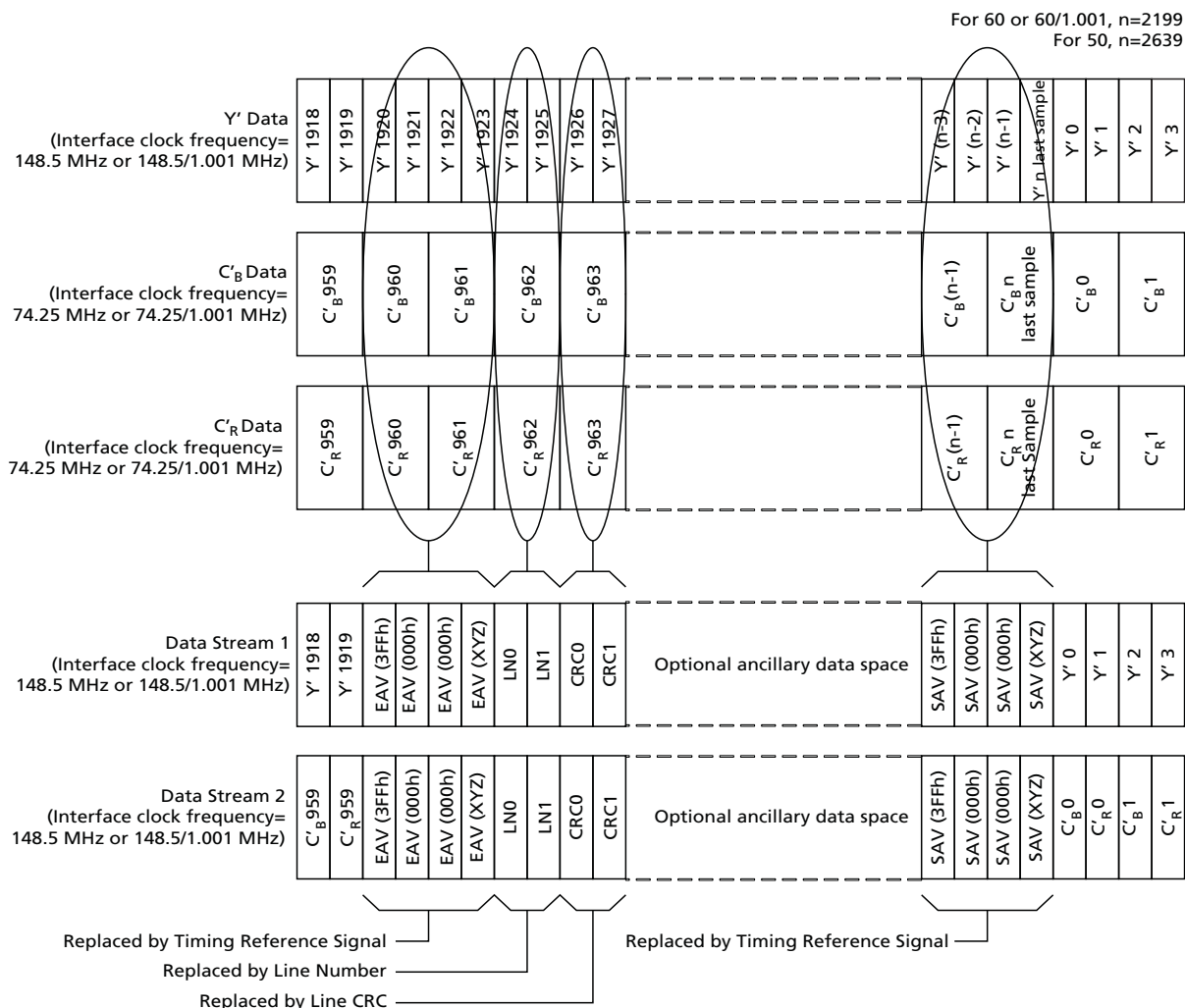
Figure 4-15: Aviaa 20-bit Mapping Structure for 1920 x 1080 50/60Hz Progressive 4:2:0 & 4:2:2 (Y'C'B'R) 8/10-bit Signals
