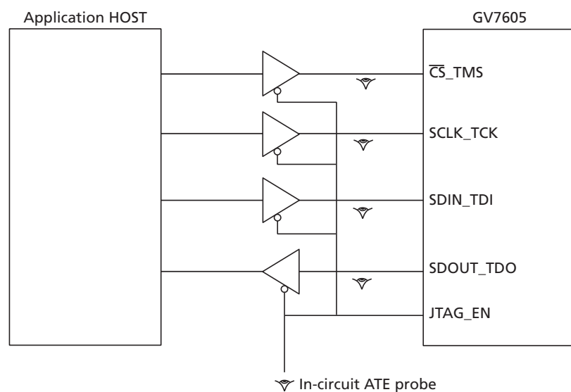
Figure 4-65: In-Circuit JTAG
