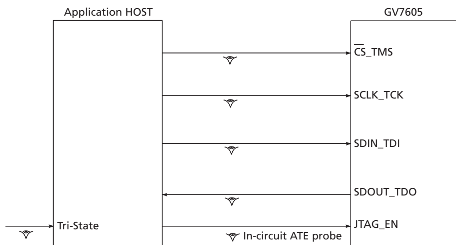
Figure 4-66: System JTAG
