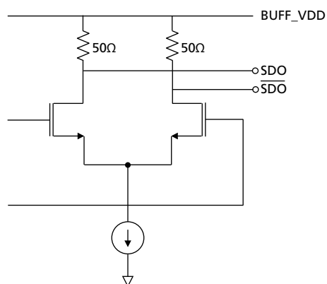
Figure 3-9: SDO/ \overline{\text{SDO}}
