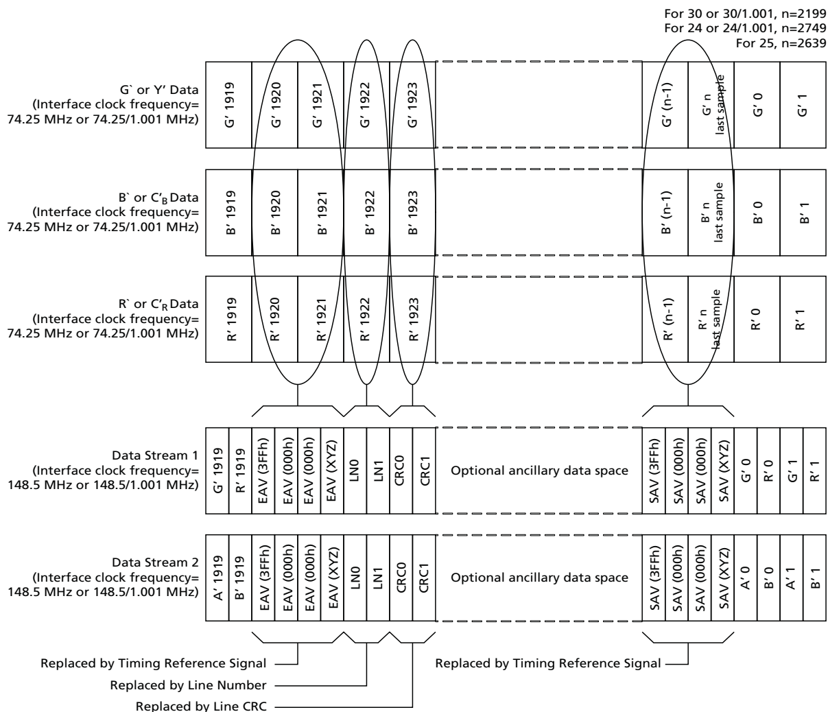
Figure 4-16: AviiA 20-bit Mapping Structure for 1920 x 1080 24/25/30Hz Progressive 4:4:4 (R'G'B') 8/10-bit Signals
