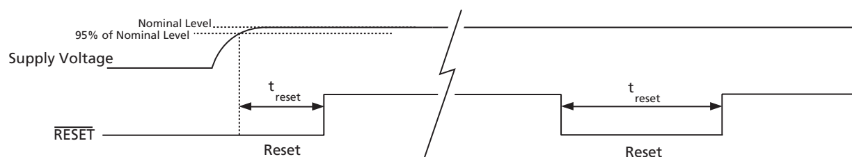
Figure 4-67: Reset Pulse
