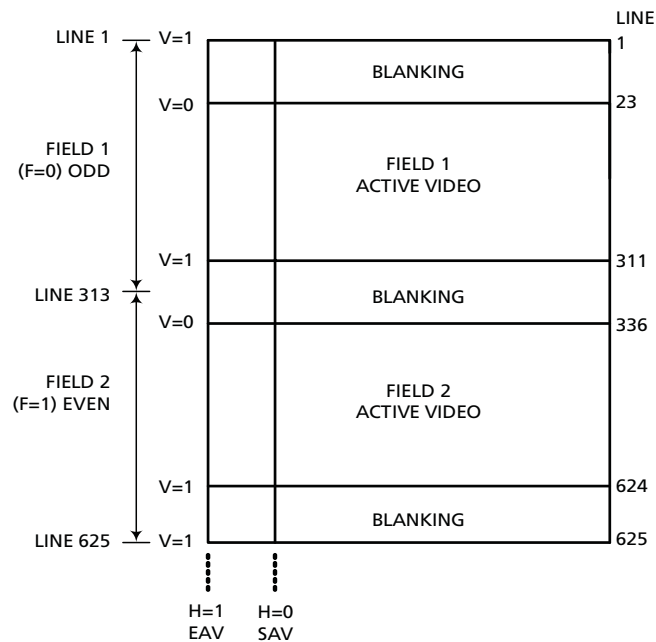
Figure 4-4: Data transmitting with blanking, 625/50Hz
