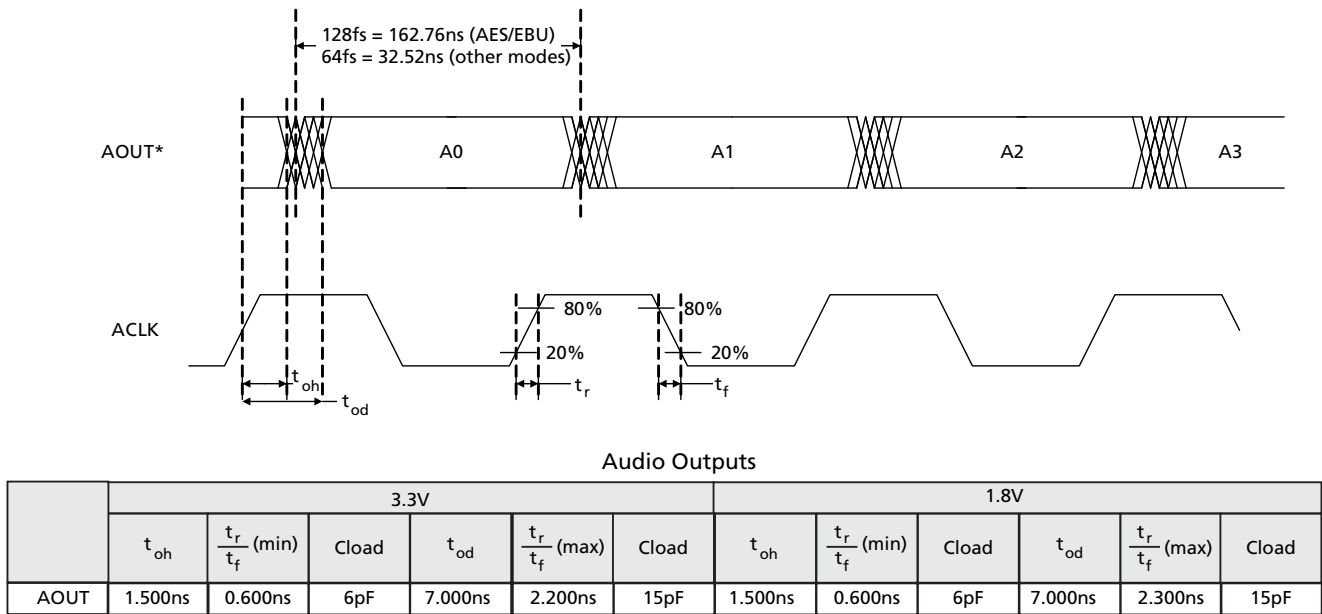
Figure 4-50: ACLK to Data and WCLK Signal Output Timing
