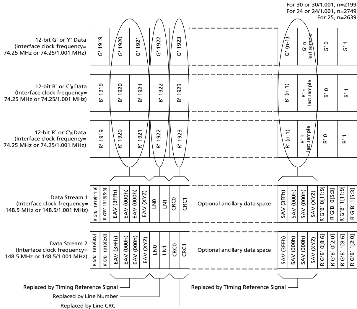
Figure 4-17: Aviaa 20-bit Mapping Structure for 1920 x 1080 24/25/30Hz Progressive 4:4:4 (R'G'B' or Y'C'B' or Y'C'R) 12-bit Signals
