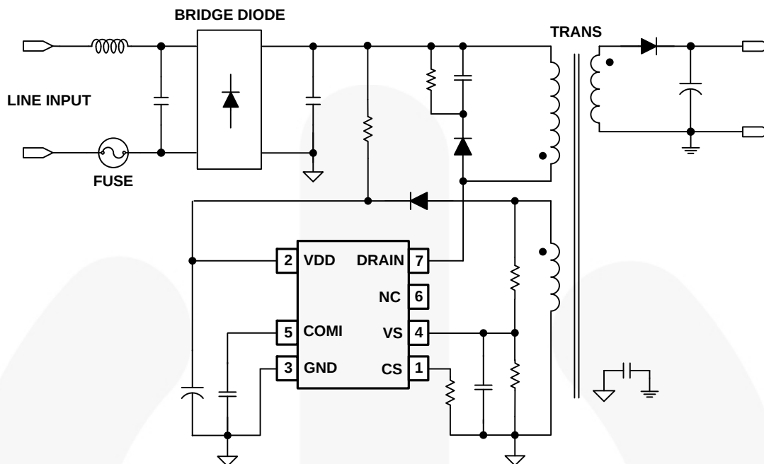
Figure 1. Typical Application
