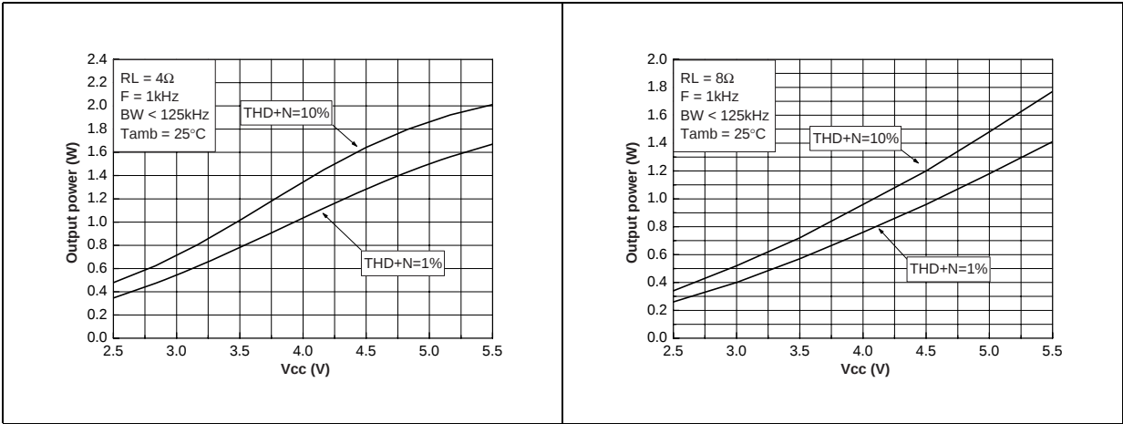
Figure 10. Output power vs. power supply voltage Figure 11. Output power vs. power supply voltage
