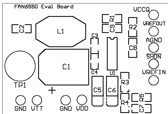
Figure 4. Top Silk
