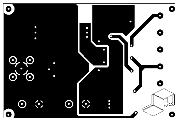
Figure 6. Bottom Layer
