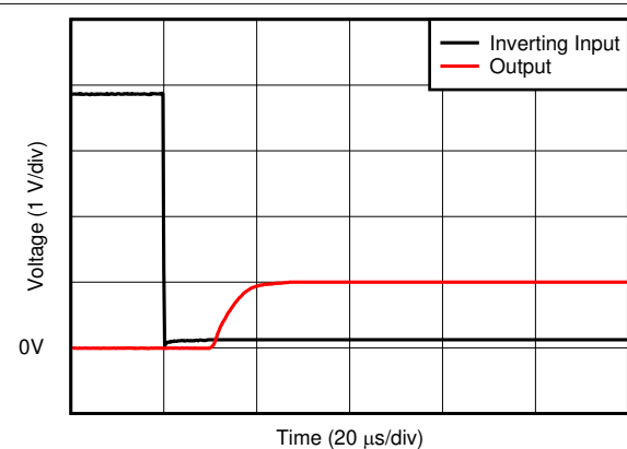
Figure 6-26. Step Response
