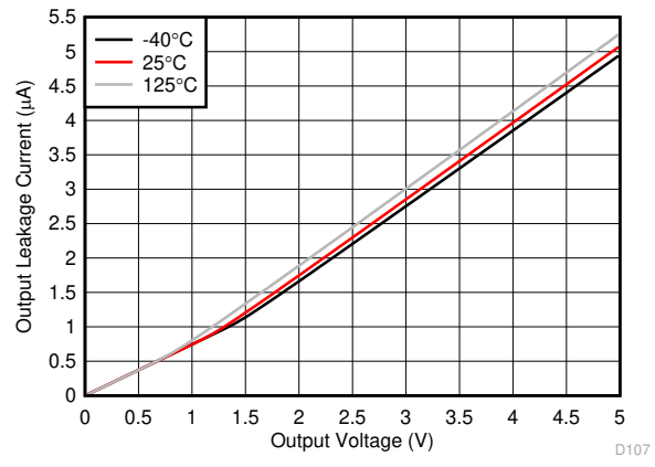
Figure 6-38. Output Leakage vs. Output Voltage
