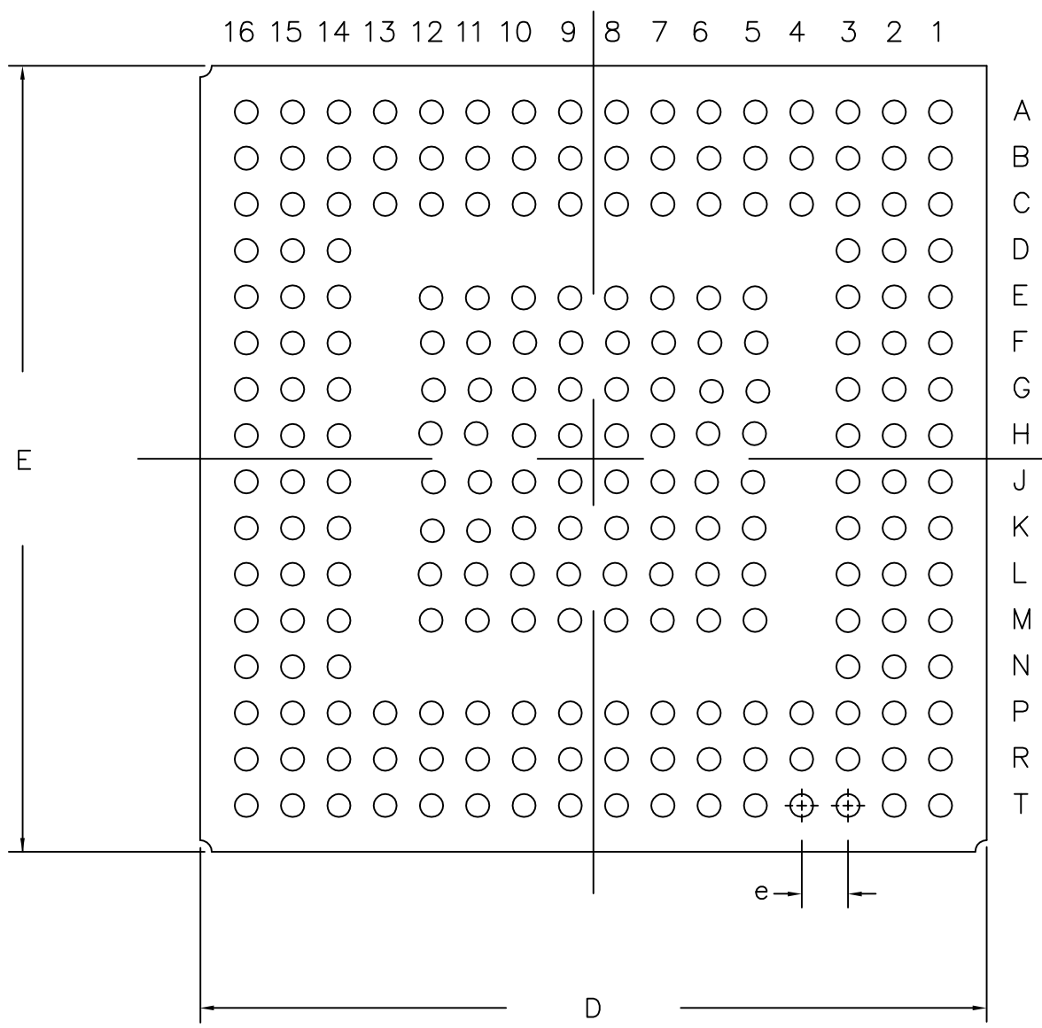
BOTTOM VIEW
