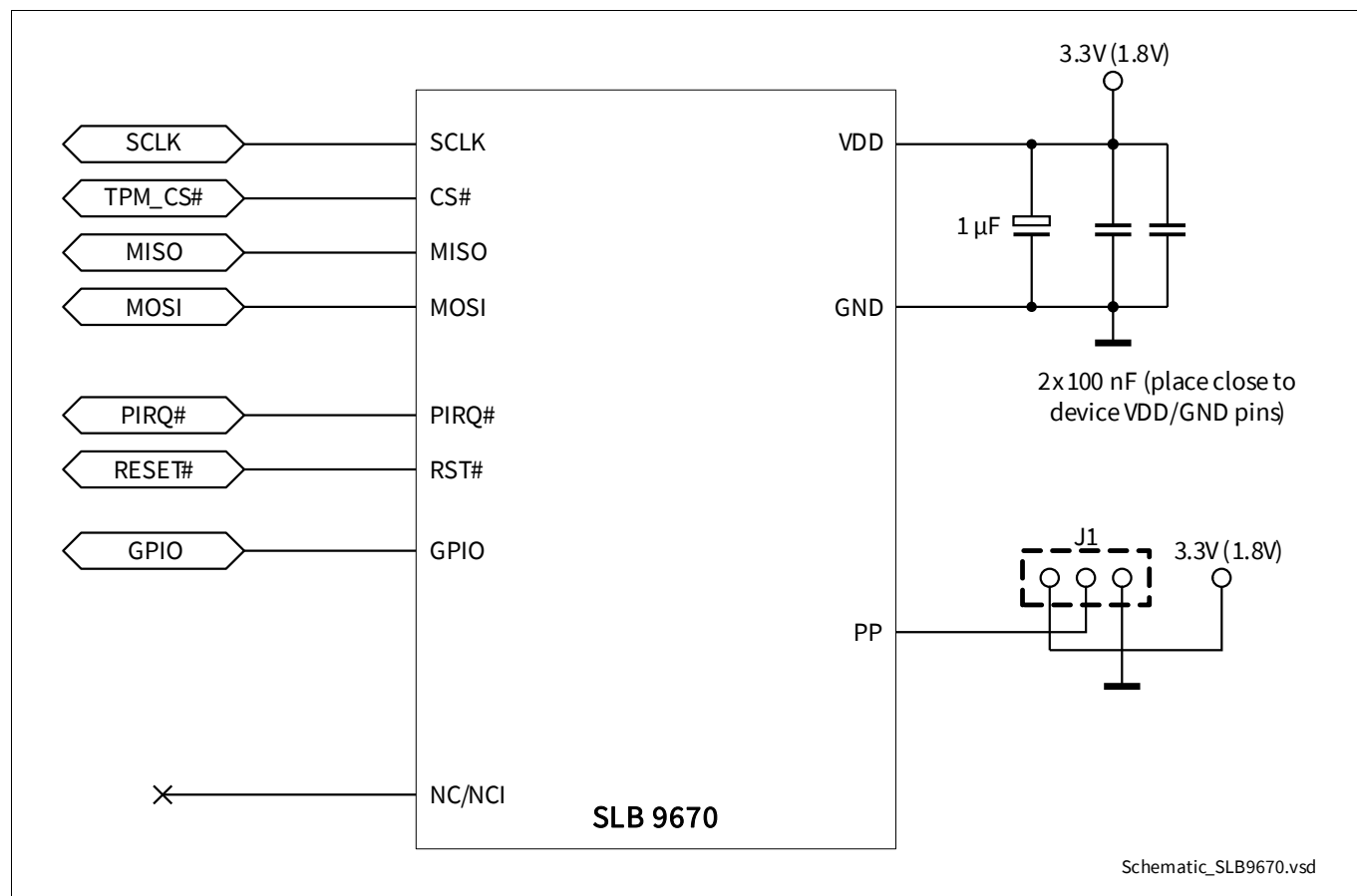
Figure 2 Typical Schematic
