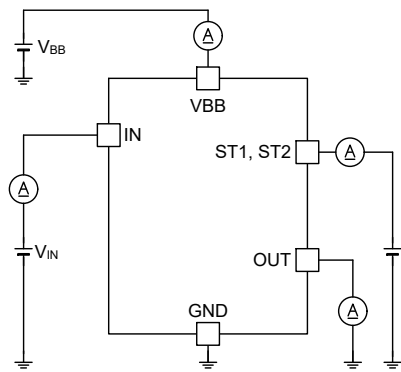
Figure 25. Standby Current Low-Level Input Current Output Leak Current Diagnostic Output Leak Current
