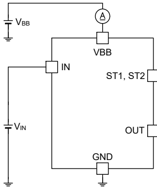
Figure 26. Operating Current
