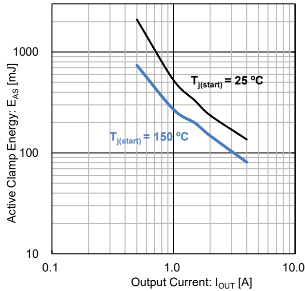
Figure 24. Active Clamp Energy vs Output Current
