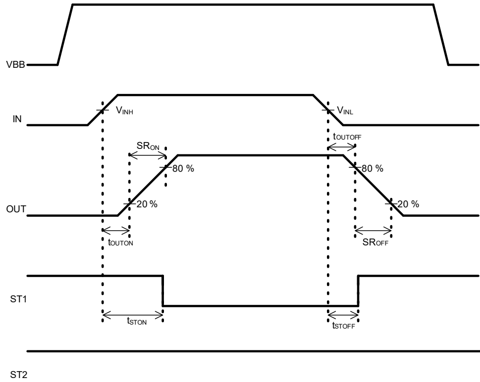
Figure 34. Timing Chart
