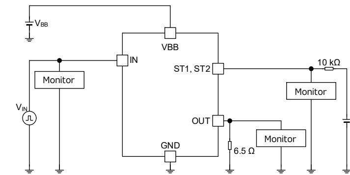
Figure 29. Output ON Slew Rate Output OFF Slew Rate Output ON Propagation Delay Time Output OFF Propagation Delay Time Diagnostic Output ON Propagation Delay Time Diagnostic Output OFF Propagation Delay Time
