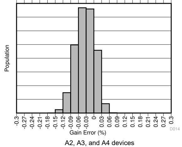
Figure 6-6. Gain Error Production Distribution
