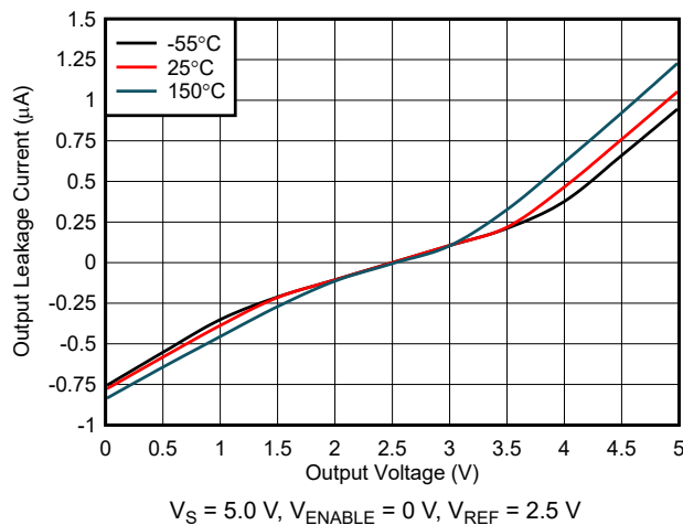
Figure 6-31. Output Leakage vs. Output Voltage (A1, A2, and A3 Devices)
