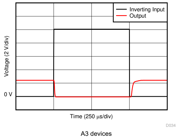
Figure 6-24. Inverting Differential Input Overload
