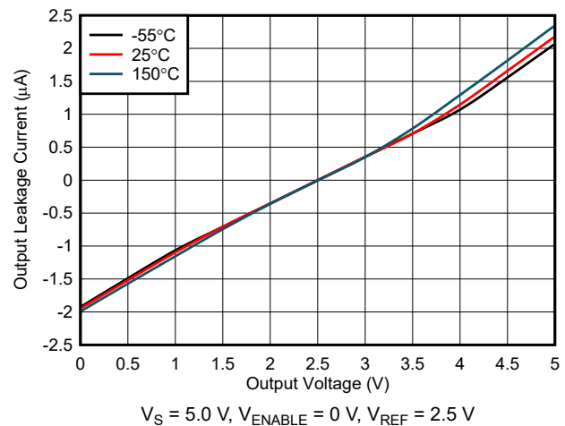
Figure 6-32. Output Leakage vs. Output Voltage (A4 and A5 Devices)
