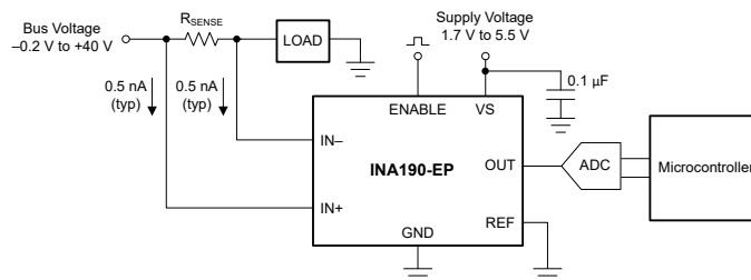
Typical Application
