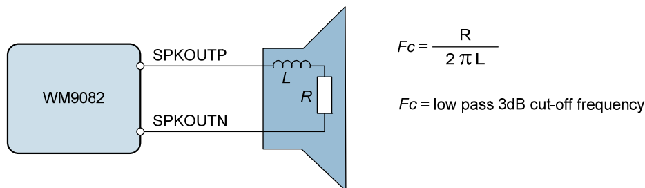
Figure 6 Speaker Equivalent Circuit for Filterless Operation
