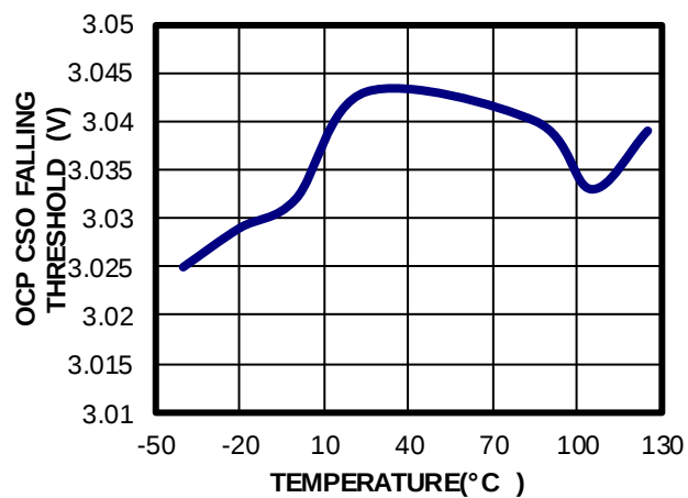
OCF CSO Falling Threshold vs. Temperature
