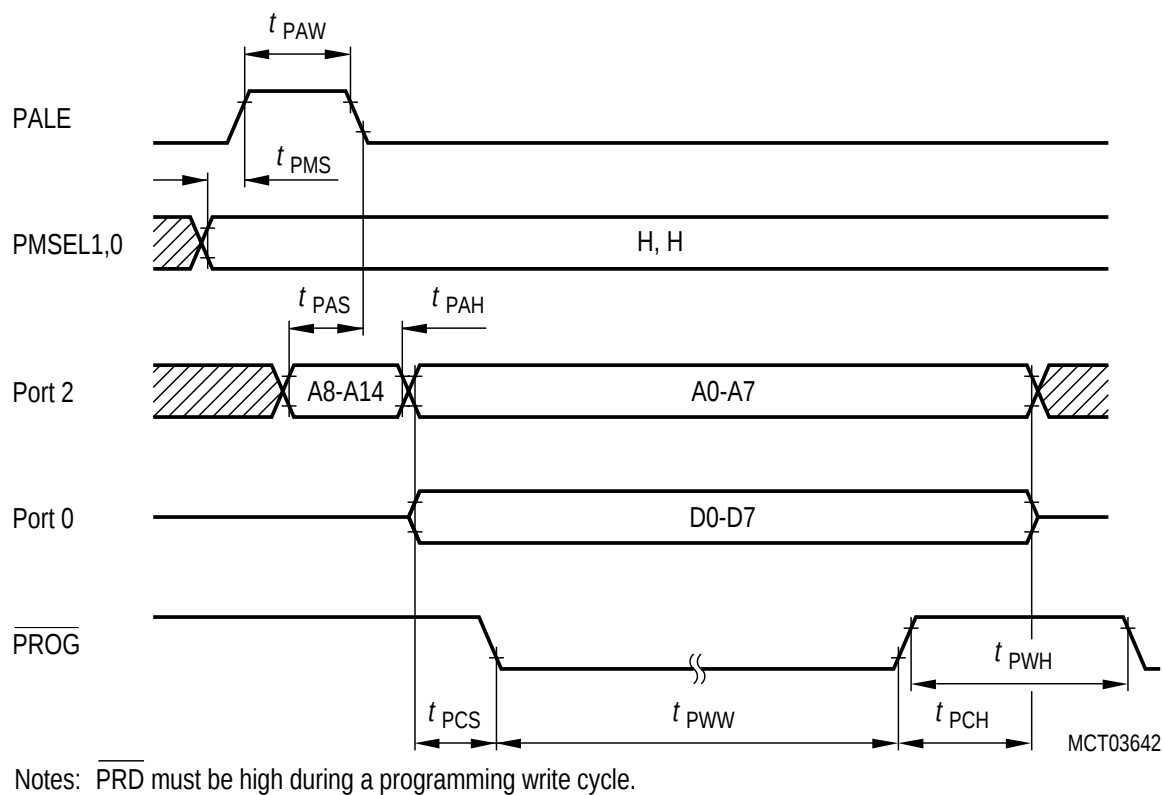
Figure 34 Programming Code Byte - Write Cycle Timing
