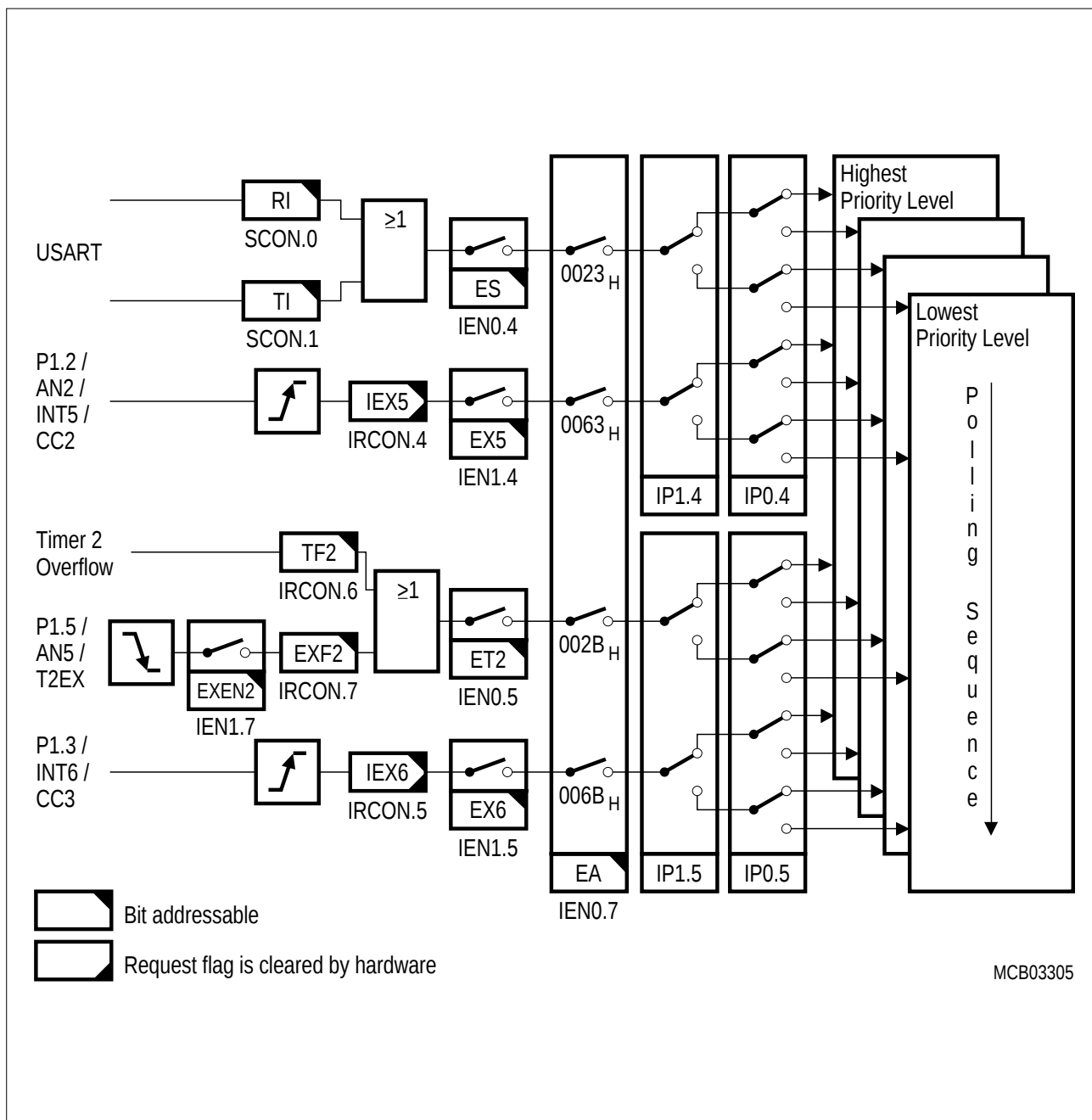
Figure 23 Interrupt Structure, Overview Part 3
