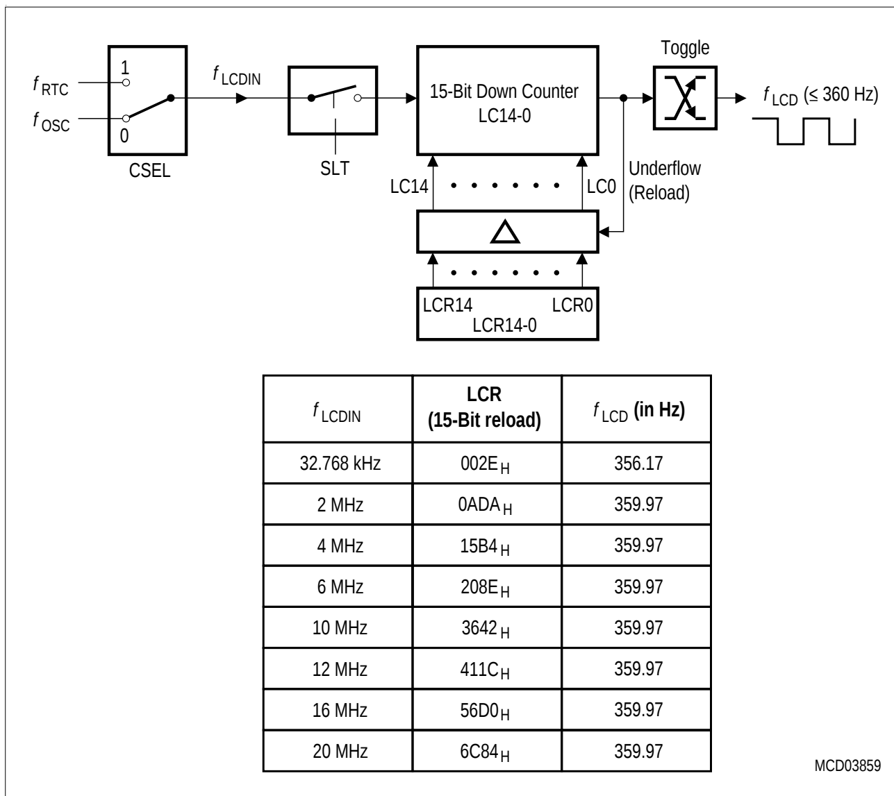
Figure 17 LCD Clocking
