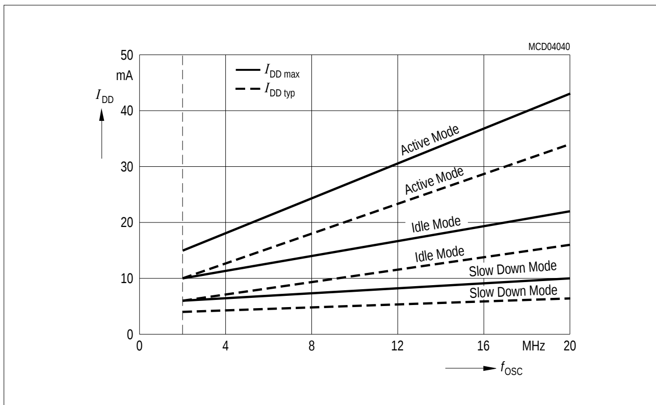
Figure 29 I_{DD} Diagram
