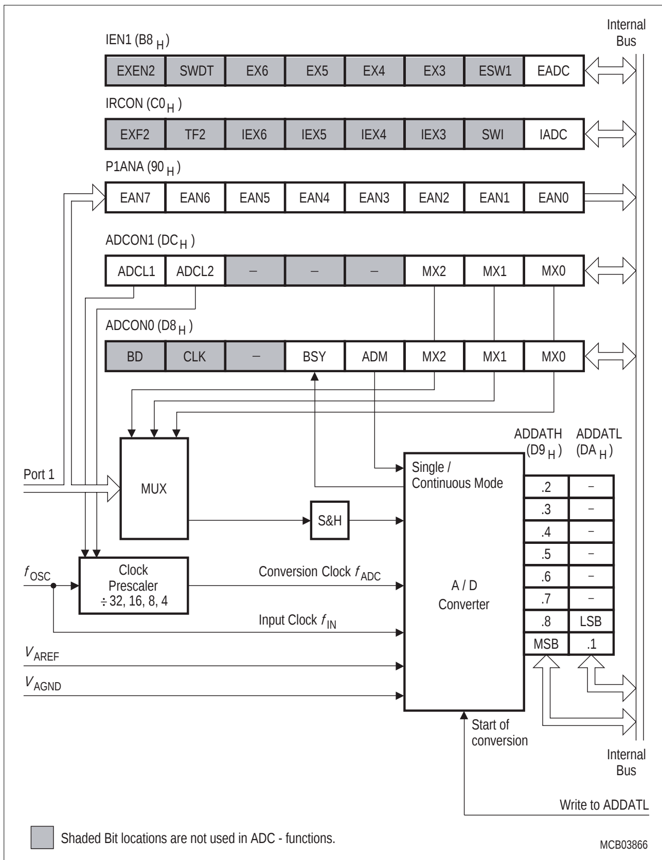
Figure 20 Block Diagram of the 10-Bit A/D Converter
