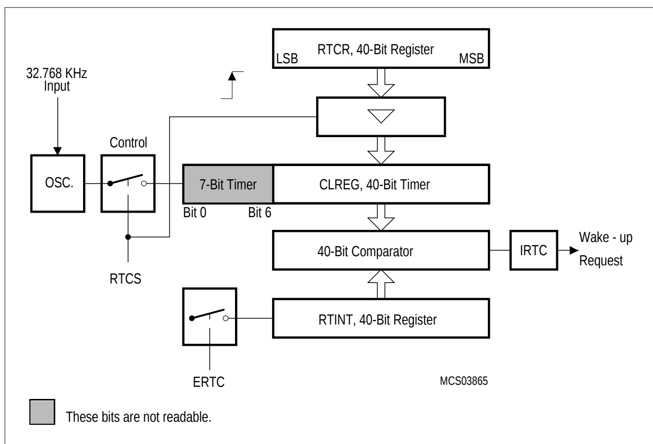
Figure 18 Real-Time Clock
