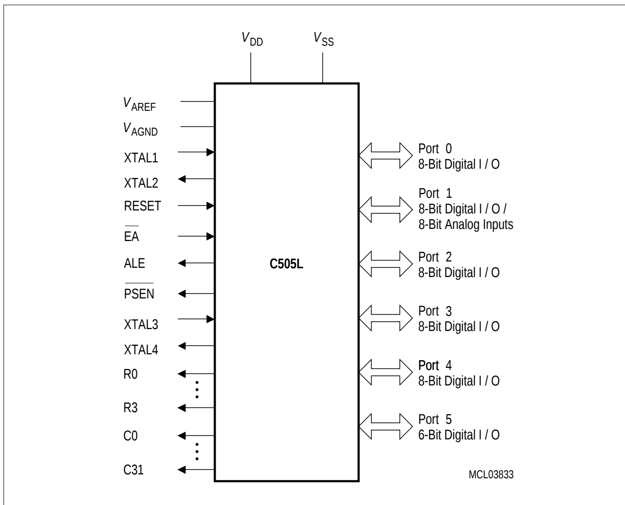
Figure 2 Logic Symbol
