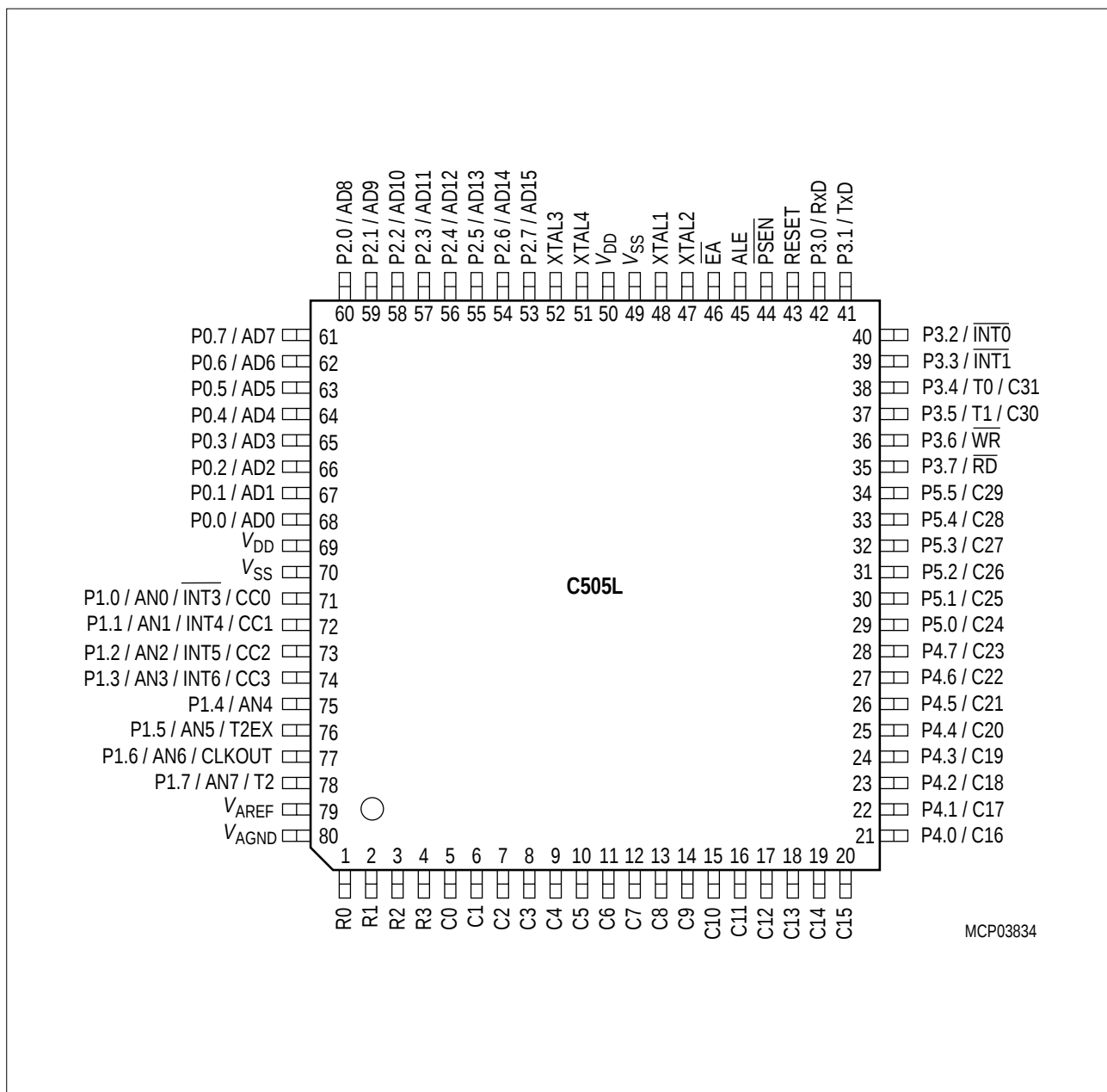
Figure 3 Pin Configuration P-MQFP-80 Package (top view)
