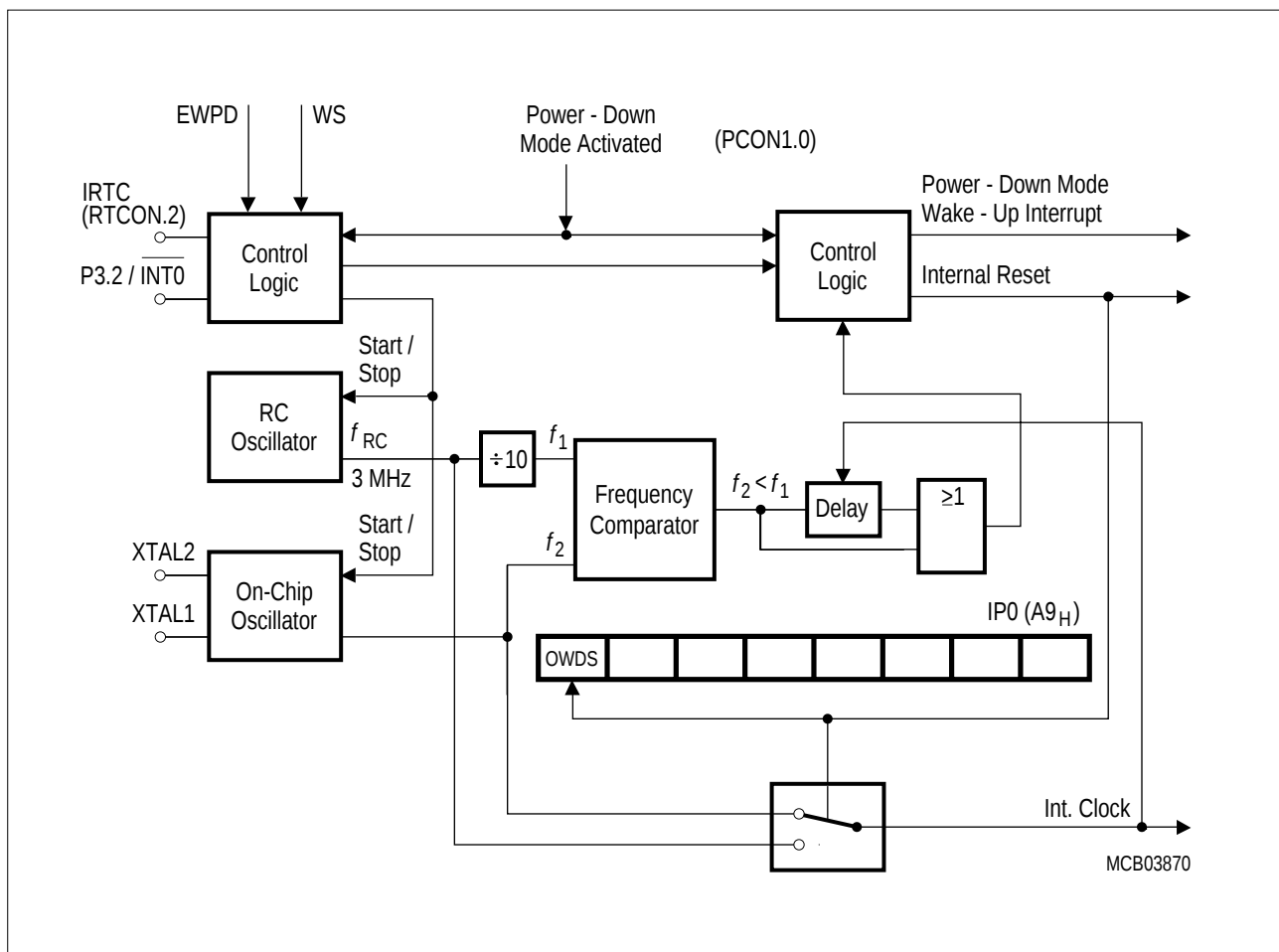
Figure 25 Block Diagram of the Oscillator Watchdog
