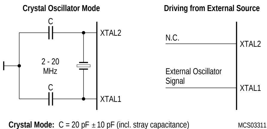
Figure 41 Recommended Oscillator Circuits for Crystal Oscillator at XTAL1
