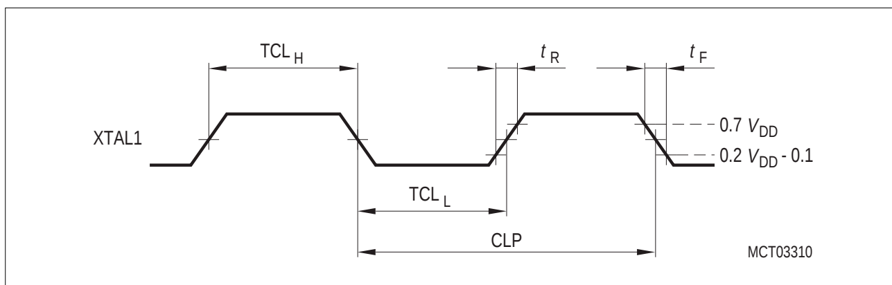
Figure 33 External Clock Drive on XTAL1
