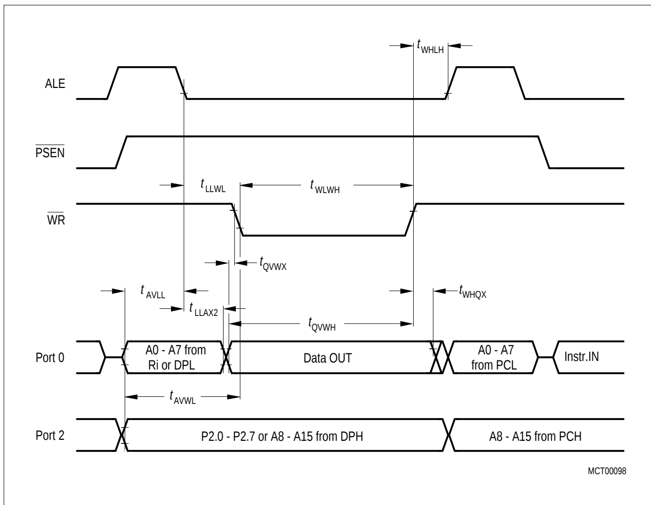
Figure 32 Data Memory Write Cycle
