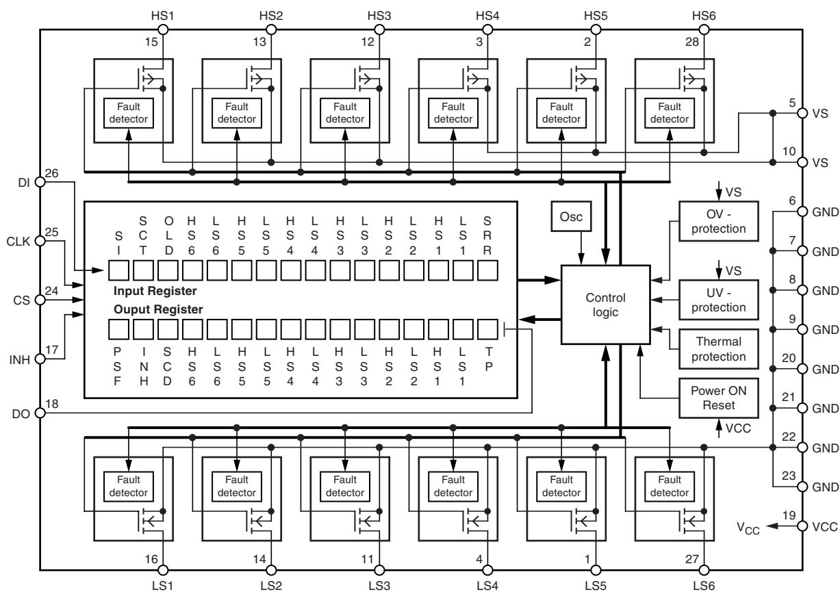
Figure 1-1. Block Diagram
