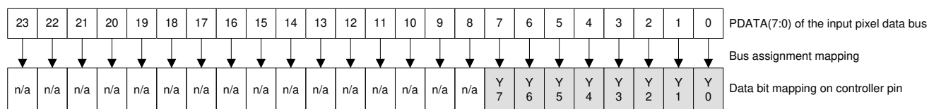
Figure 6-9. BT.656 Interface Mode Bit Mapping
