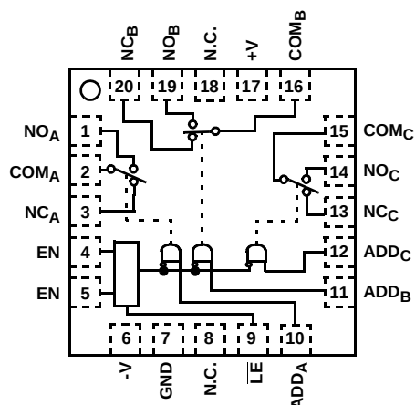
ISL43231 (QFN) TOP VIEW
