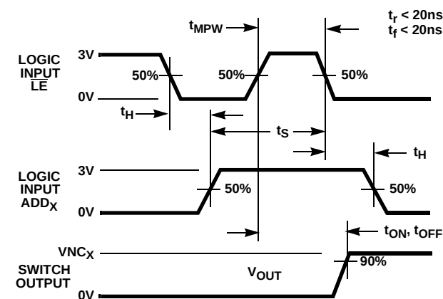
FIGURE 3. BREAK-BEFORE-MAKE TIME
