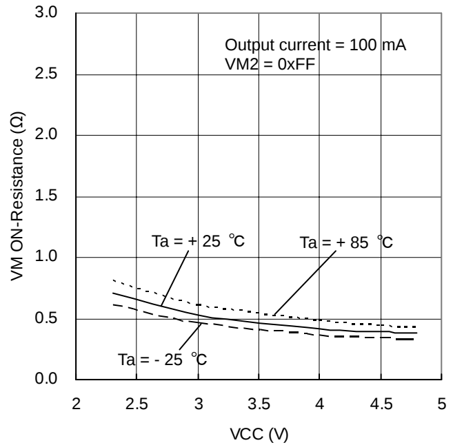
Figure 5. VM ON-Resistance
