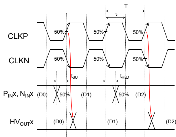
Figure 2 LVDS/CMOS CLK mode ( \text{CLKEN}=0 )
