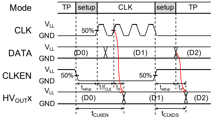
Figure 9 Clock enable/disable time
