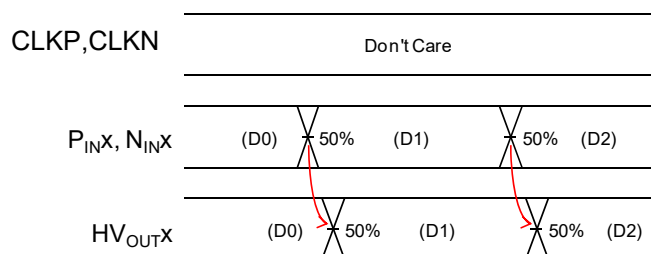
Figure 3 TP mode ( \text{CLKEN}=1 )
