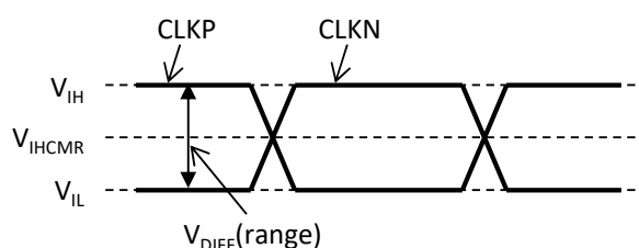
Figure 4 Differential input voltage range ( V_{DIFF}(\text{range}) )
