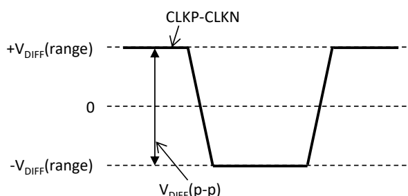
Figure 5 Differential input voltage peak to peak swing ( V_{DIFF}(\text{p-p}) )
