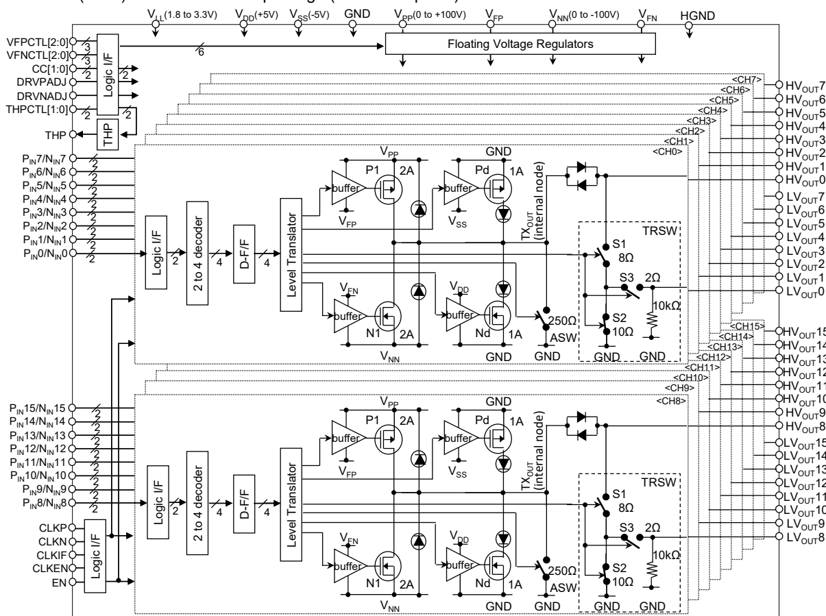
Figure 1 Block Diagram
