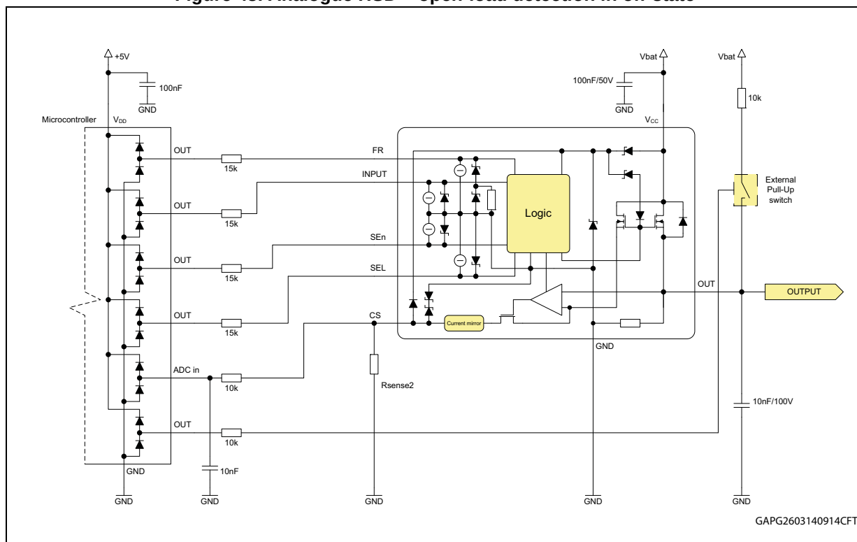
Figure 43. Analogue HSD – open-load detection in off-state
