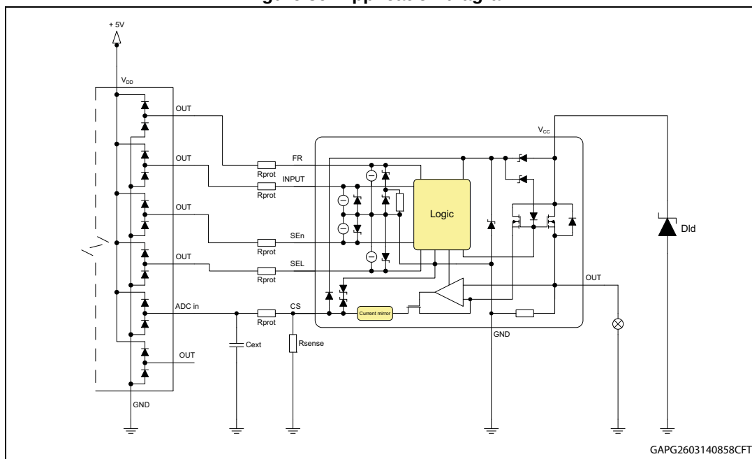
Figure 39. Application diagram
