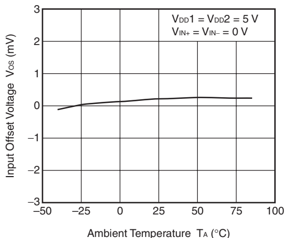
INPUT OFFSET VOLTAGE vs. AMBIENT TEMPERATURE
