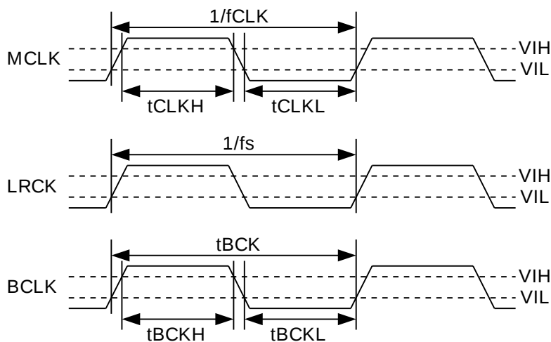
Figure 2. Clock Timing
