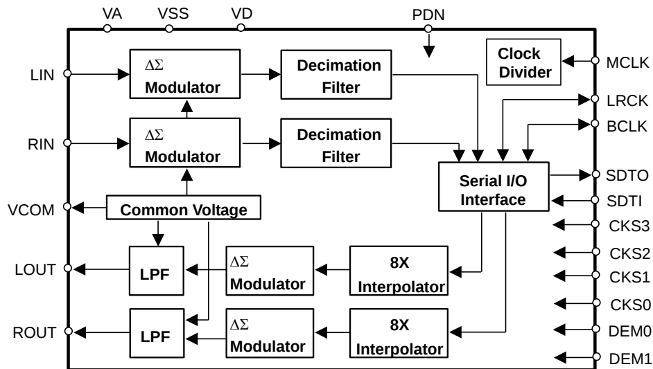
Figure 1. Block Diagram
