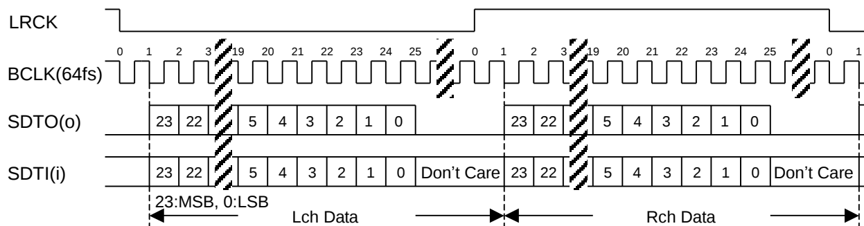
Figure 7. Mode I²S Timing
