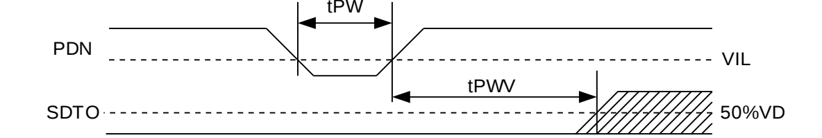
Figure 5. Reset Timing
