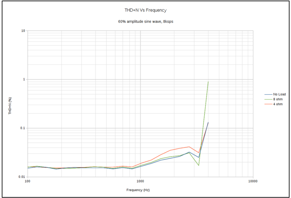
Figure 62 Class D amplifier THD+N vs. Frequency 8ksps
