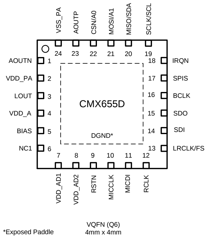
Figure 6 CMX655D Pin Arrangement
