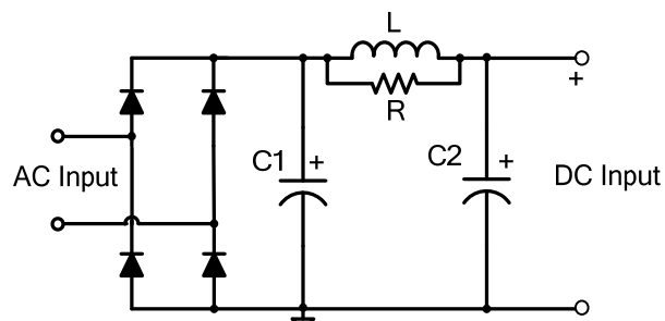
Figure 11: Input Filter
