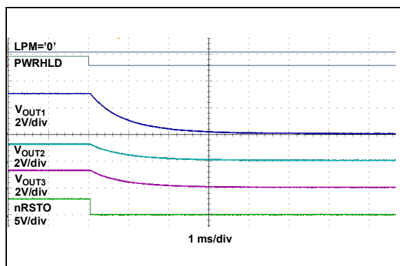
FIGURE 2-14: PWRHLD Shutdown Sequence.
