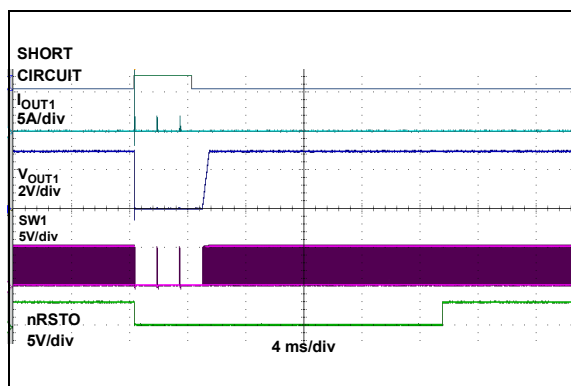
FIGURE 2-17: Output Short Circuit on V_{OUT1} .
