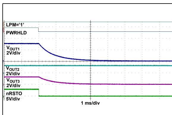
FIGURE 2-15: Entering Hibernate Mode.
