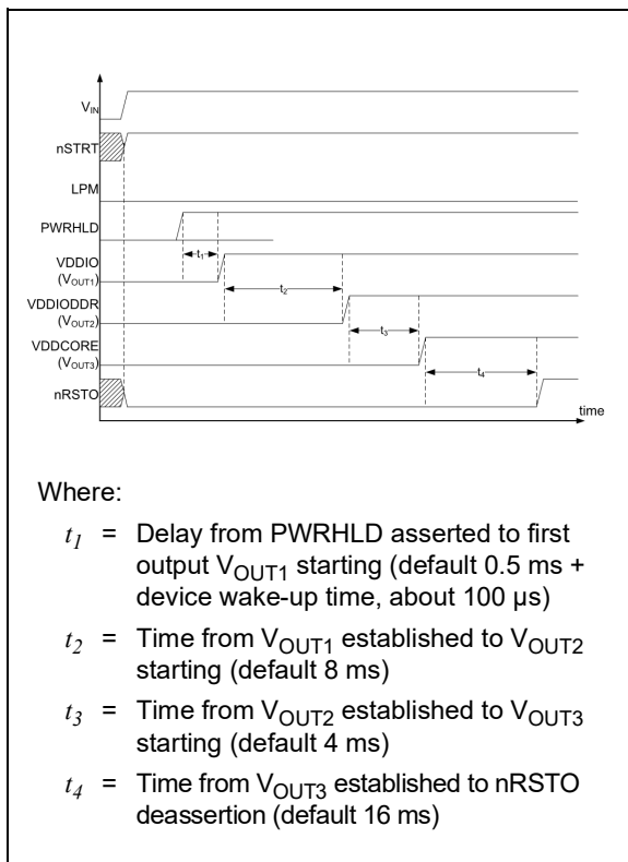
FIGURE 4-5: Start-Up from PWRHLD Timing Diagram.
