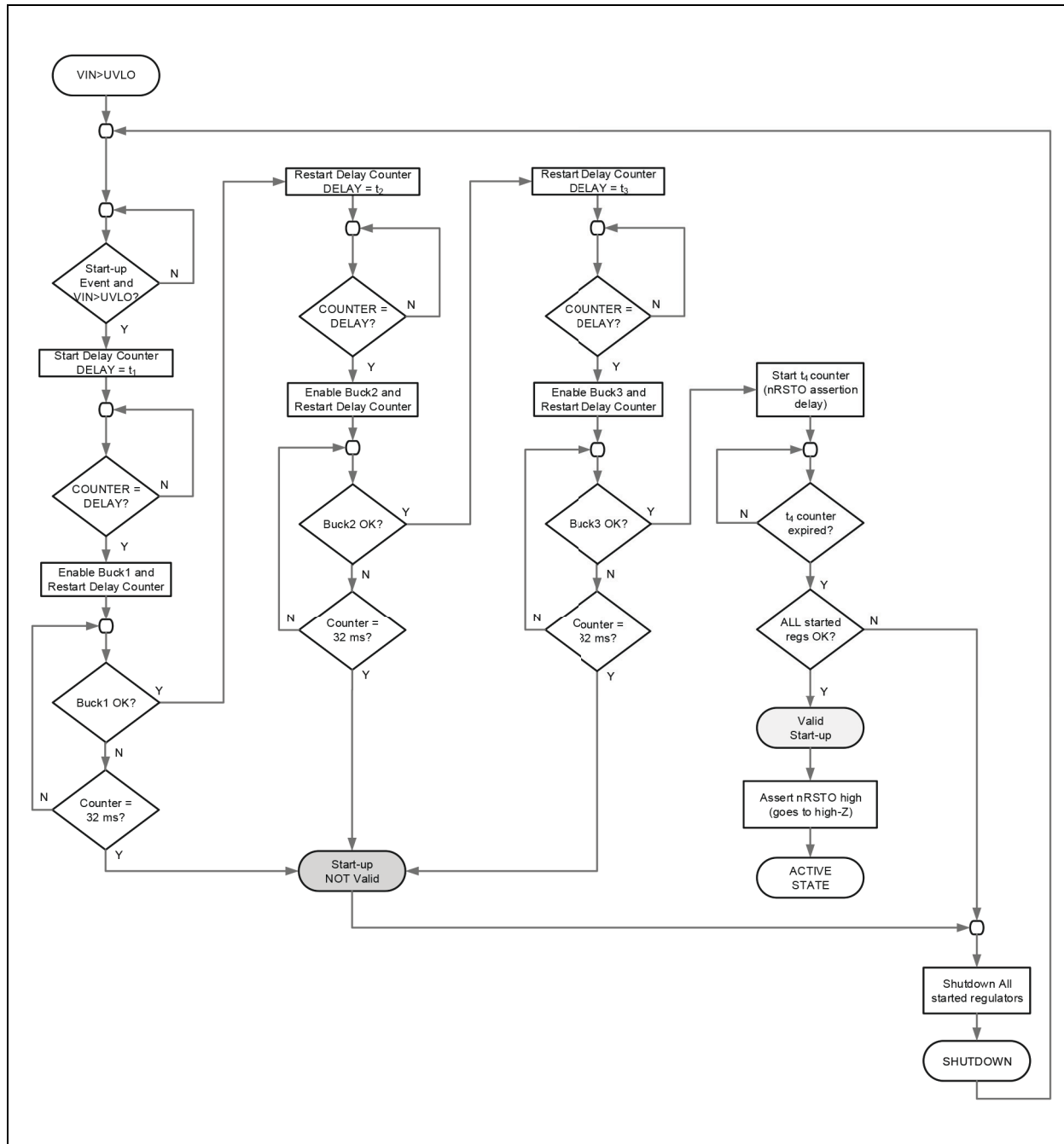
FIGURE 4-6: Start-up Sequence Flowchart.
