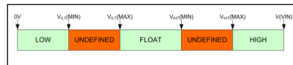
FIGURE 4-3: SELVx High, Low and Float States Threshold.
