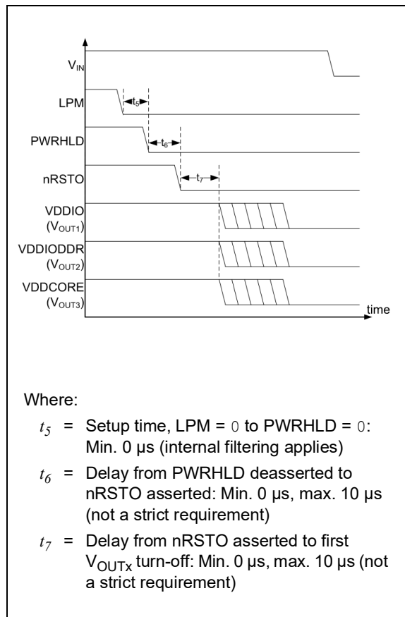
FIGURE 4-7: Power-Down (Shutdown) Sequence Timing Diagram.
