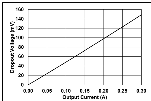
FIGURE 2-11: LDO Dropout Voltage vs. Load Current.
