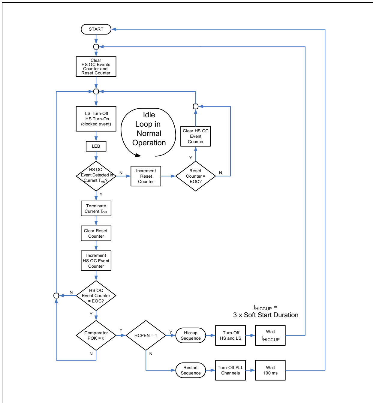
FIGURE 5-1: Hiccup Mode Protection Flowchart.
