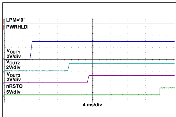
FIGURE 2-13: PWRHLD Start-up Sequence.
