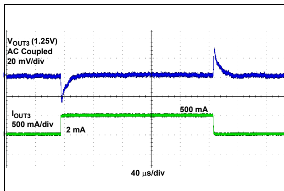
FIGURE 2-16: Buck3 Transient Response (Active Mode, V_{OUT3} = 1.25V ).
