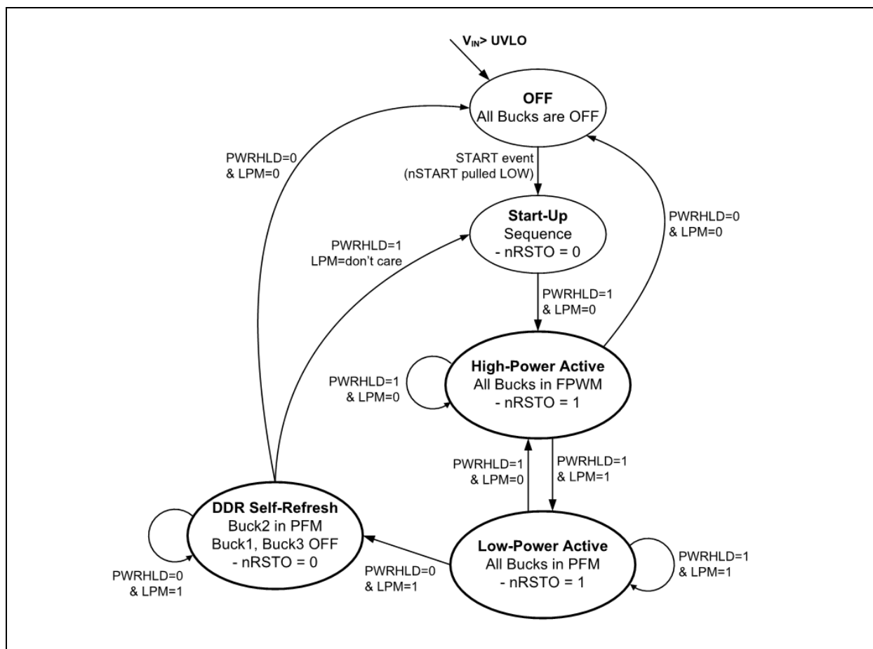
FIGURE 4-2: Finite State Machine (FSM) States Diagram for MCP16501.
