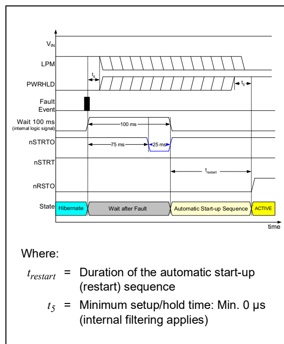
FIGURE 4-10: Automatic Wake-Up Pulse Generation Timing Diagram (Fault during Hibernate).
