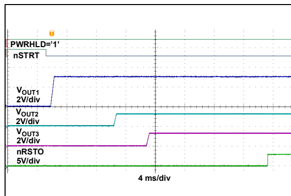
FIGURE 2-12: nSTRT Start-up Sequence.
