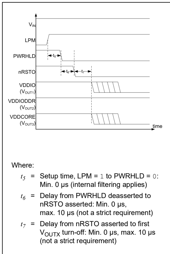
FIGURE 4-8: Entering Hibernate Mode Timing Diagram.
