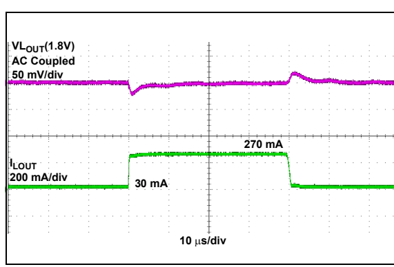
FIGURE 2-18: LDO Load Transient Response.
