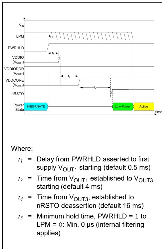
FIGURE 4-9: Start-up Sequence Exiting Hibernate Mode Timing Diagram.
