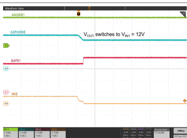
Figure 9-16. ORing V_{IN2} to V_{IN1} Switch Over
