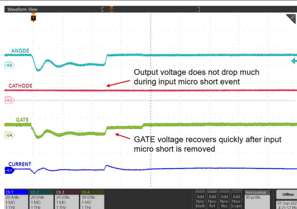
Figure 9-9. Response to LV124 E-10 (Input Micro Short, 100 \mu s)
