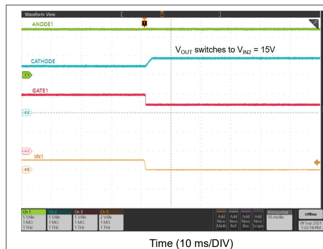
Figure 9-13. ORing V_{IN1} to V_{IN2} Switch Over
