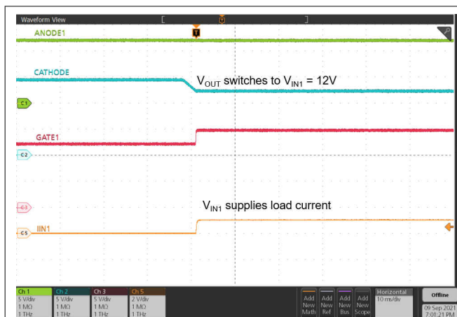
Figure 9-15. ORing V_{IN2} to V_{IN1} Switch Over
