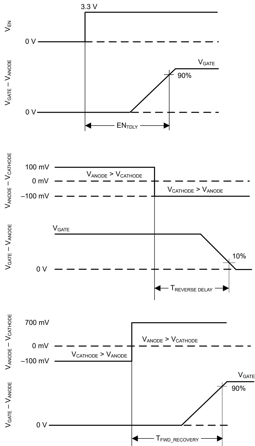
Figure 7-1. Timing Waveforms
