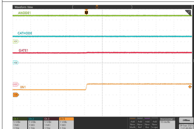
Figure 9-15. ORing V_{IN2} to V_{IN1} Switch Over
