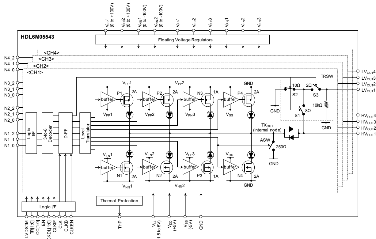
Fig.1 Block diagram
