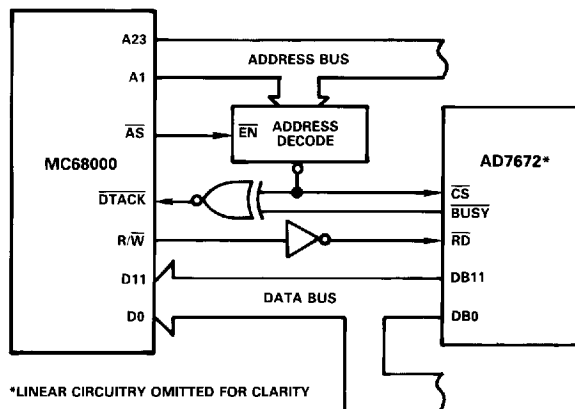
Figure 18. AD7672 - MC68000 Interface
