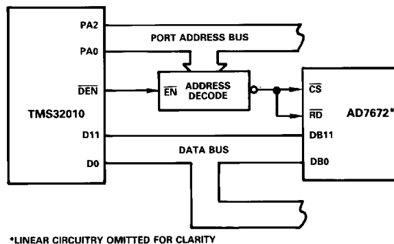
Figure 22. AD7672 - TMS32010 Interface
