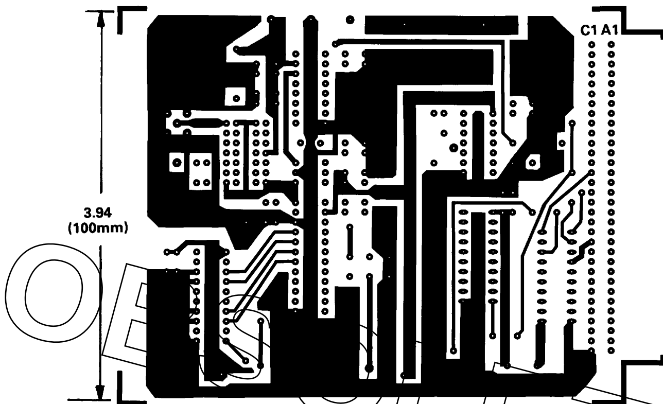
Figure 29. PCB Component Side Layout for Figure 24
