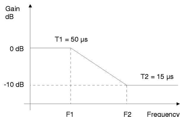
Figure 14. De-emphasis Curve.
