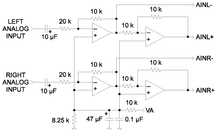
Figure 6. Optional Line Input Buffer
