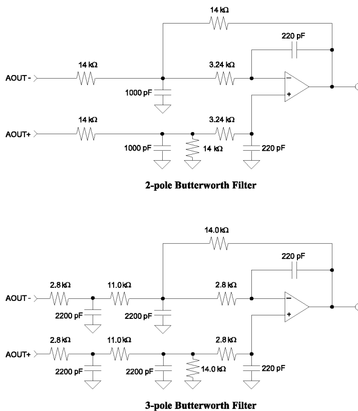
Figure 9. 2- and 3-Pole Butterworth Filters
