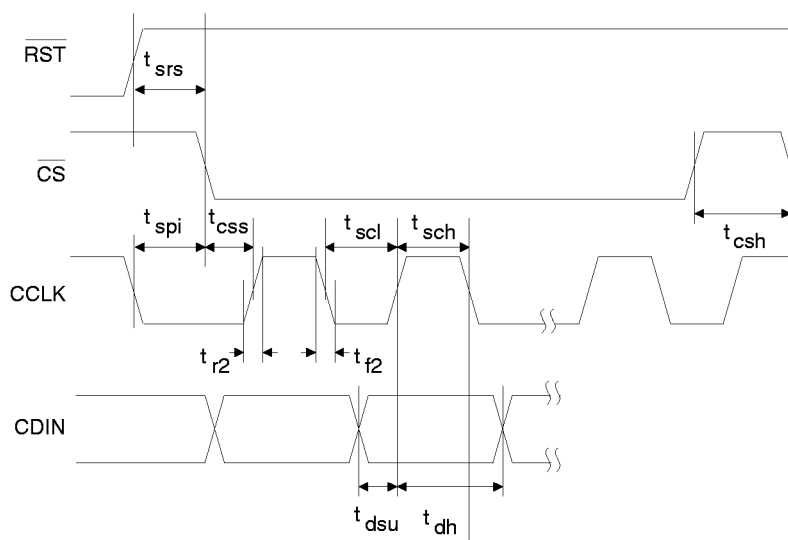
Figure 2. SPI Control Port Timing
